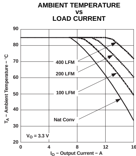
Figure 5. Safe Operating Area
