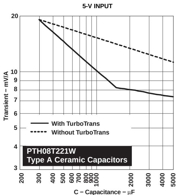
Figure 14. Capacitor Type A, 100 ≤ C(μF)×ESR(mΩ) ≤ 1000 (e.g. Ceramic)
