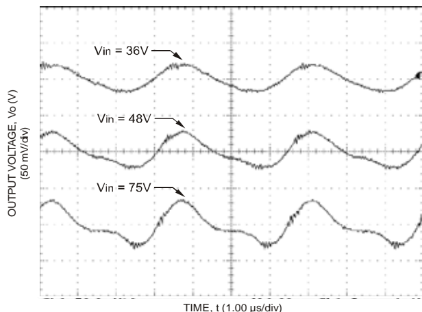
Figure 3. Output Ripple Voltage ( I_O = I_{O, \text{max}} ).
