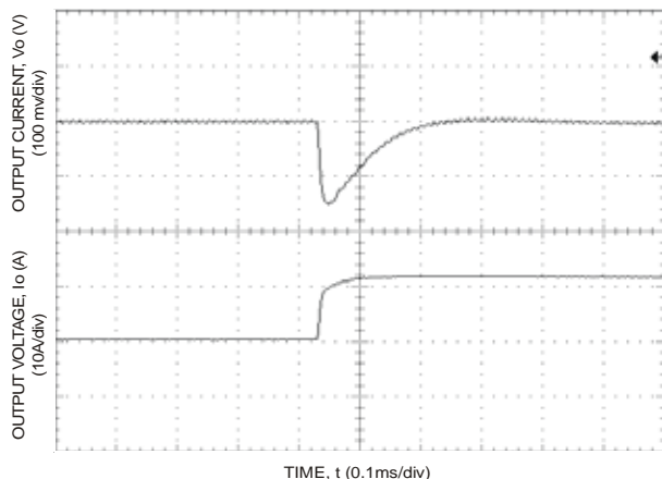
Figure 5. Transient Response to Step Increase in Load from 50% to 75% of Full Load ( V_I = 48\text{ Vdc} ).
