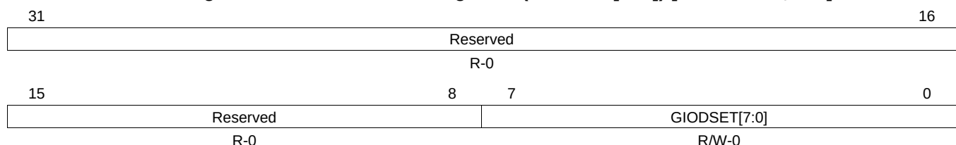
Figure 22-20. GIO Data Set Registers (GIODSET[A-B]) [offset = 40h, 60h]
