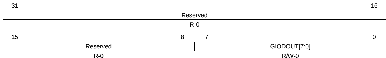
Figure 22-19. GIO Data Output Registers (GIODOUT[A-B]) [offset = 3Ch, 5Ch]
