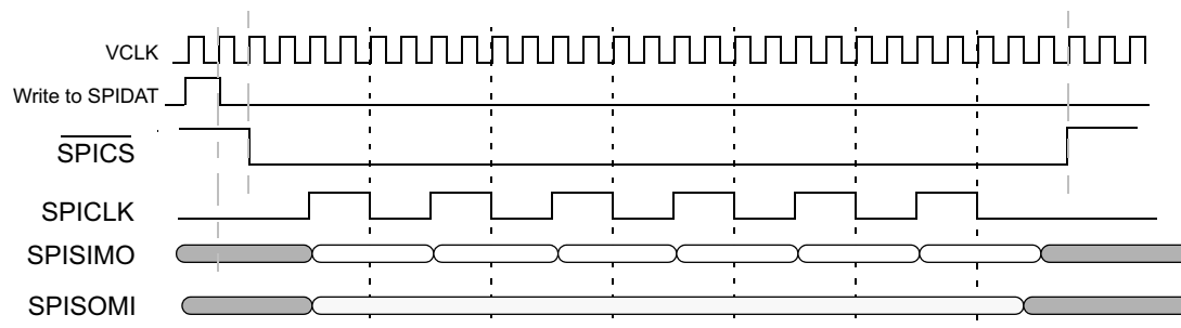
Figure 24-82. SPI/MibSPI Pins During Master Mode 4-pin with \overline{\text{SPIC}}\overline{\text{S}} Configuration
