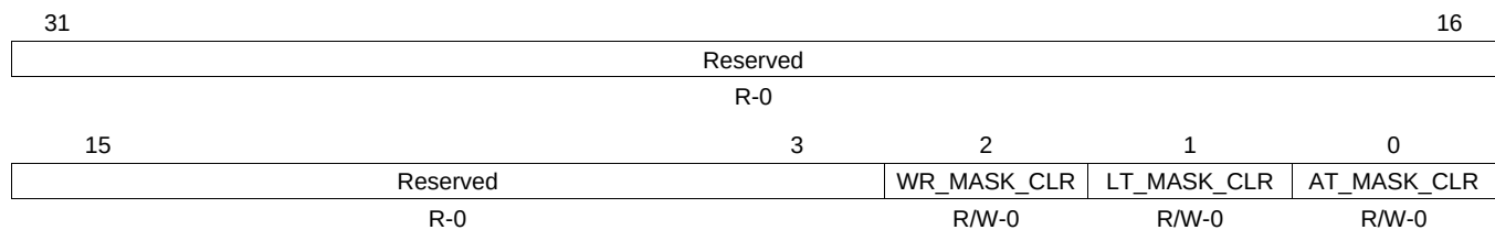
Figure 17-25. EMIF Interrupt Mask Clear Register (INTMSKCLR) [offset = 4Ch]
