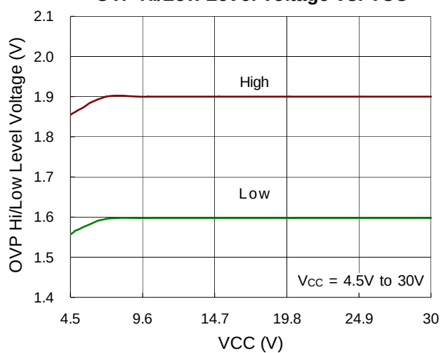
OVP Hi/Low Level Voltage vs. VCC
