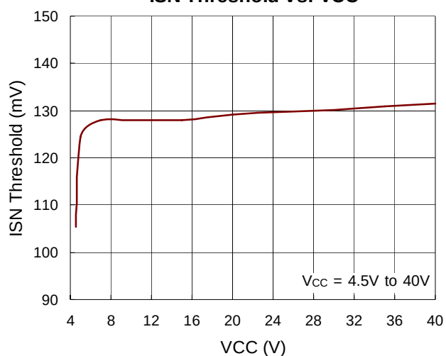
ISN Threshold vs. VCC
