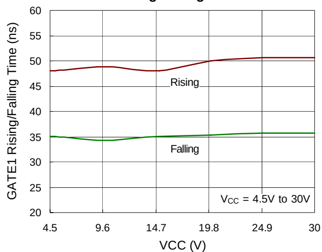
GATE1 Rising/Falling Time vs. VCC
