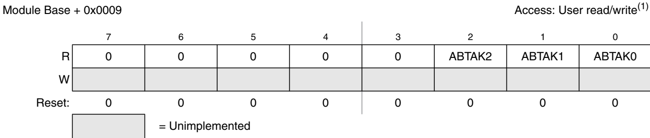
Figure 16-13. MSCAN Transmitter Message Abort Acknowledge Register (CANTAABK)
