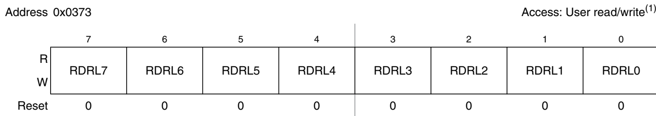
Figure 2-94. Port L Reduced Drive Register (RDRL)
