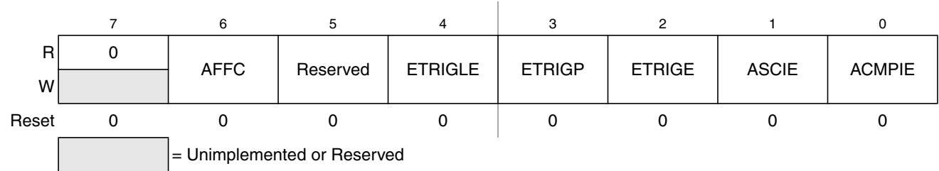
Figure 11-5. ATD Control Register 2 (ATDCTL2)
