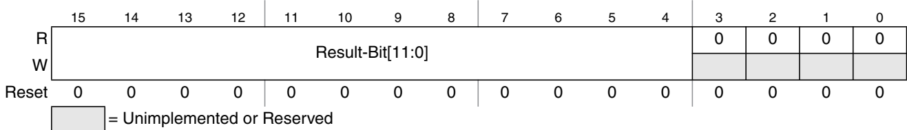
Figure 14-14. Left justified ATD conversion result register (ATDDRn)
