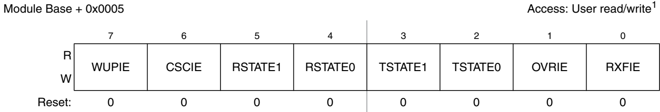
Figure 18-9. MSCAN Receiver Interrupt Enable Register (CANRIER)
