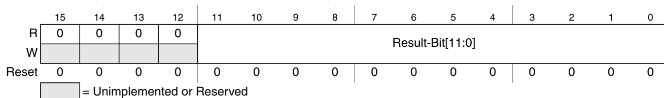
Figure 15-15. Right justified ATD conversion result register (ATDDR n )
