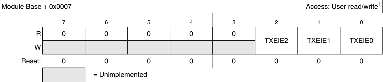
Figure 18-11. MSCAN Transmitter Interrupt Enable Register (CANTIER)
