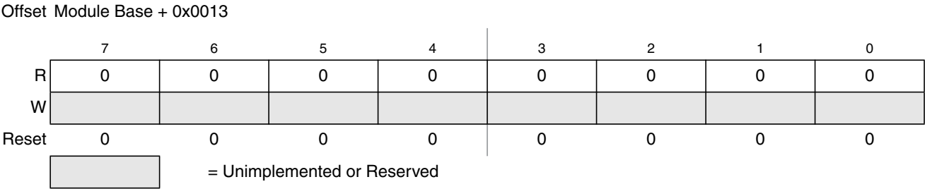
Figure 28-25. Flash Reserved7 Register (FRSV7)
