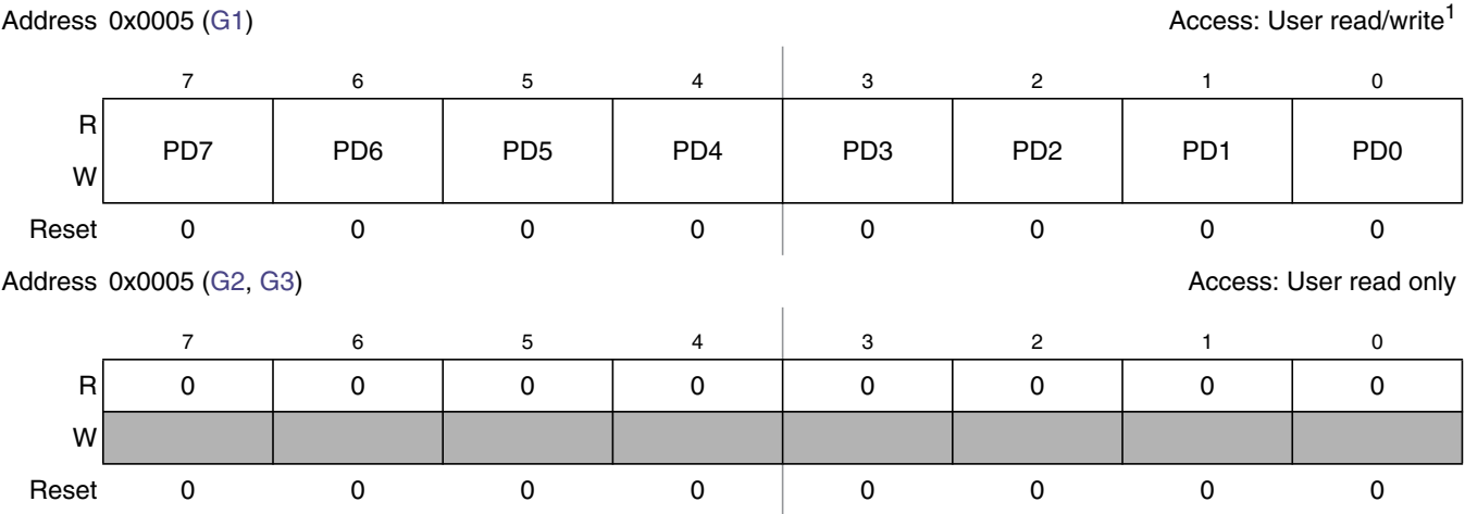
Figure 2-7. Port D Data Register (PORTD)
