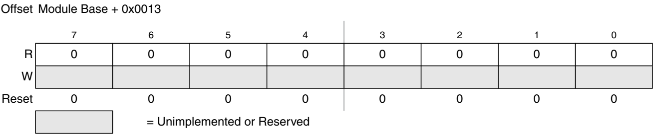
Figure 25-25. Flash Reserved7 Register (FRSV7)
