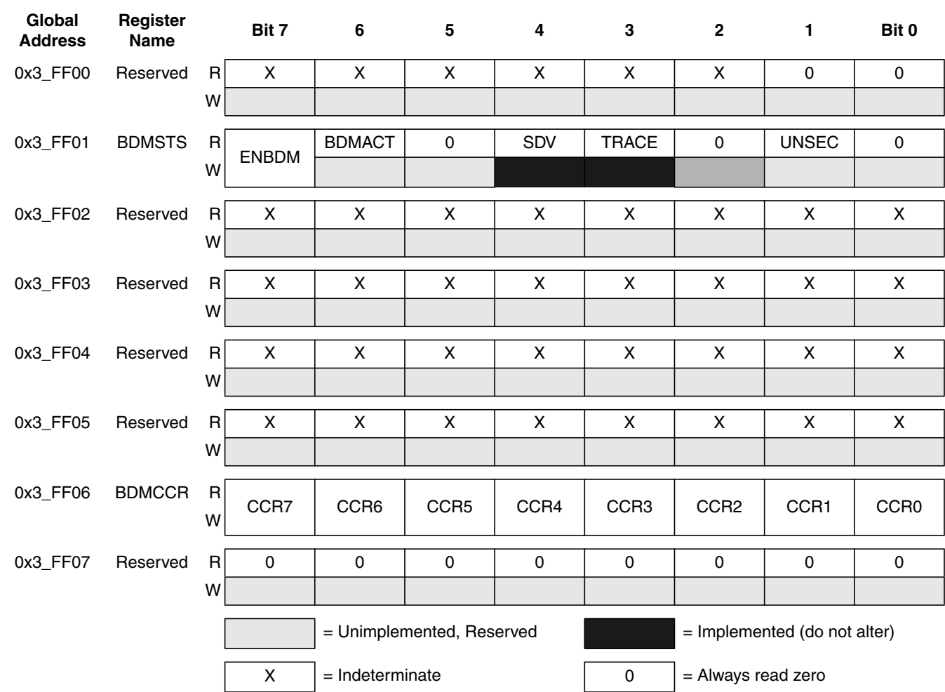
Figure 7-2. BDM Register Summary
