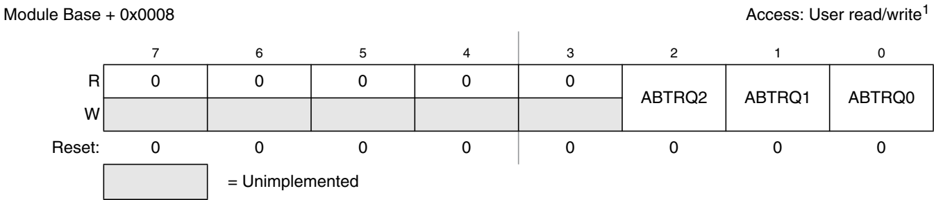
Figure 18-12. MSCAN Transmitter Message Abort Request Register (CANTARQ)
