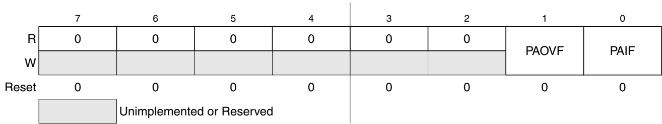
Figure 23-25. Pulse Accumulator Flag Register (PAFLG)
