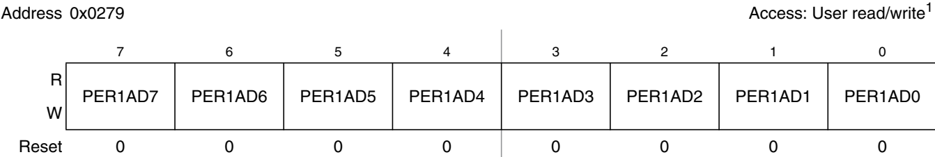
Figure 2-57. Port AD Pullup Enable Register (PER1AD)
