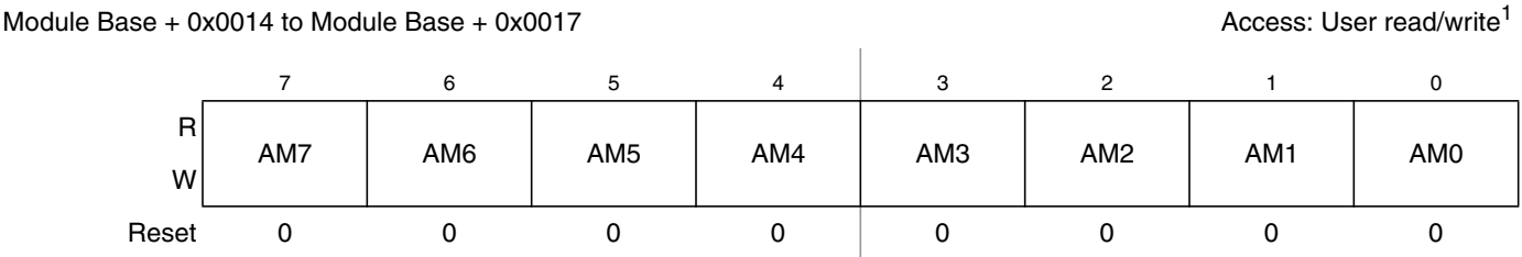
Figure 18-22. MSCAN Identifier Mask Registers (First Bank) — CANIDMR0–CANIDMR3
