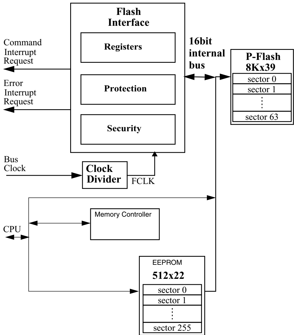
Figure 25-1. FTMRG32K1 Block Diagram
