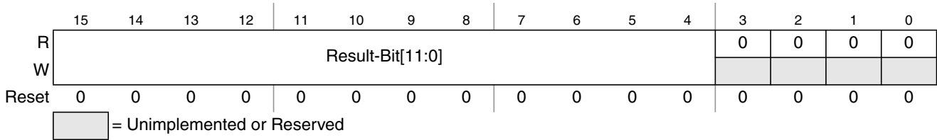
Figure 15-14. Left justified ATD conversion result register (ATDDRn)
