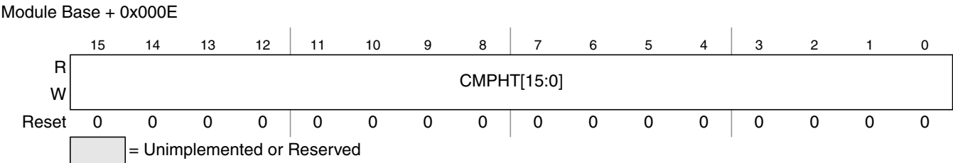
Figure 15-13. ATD Compare Higher Than Register (ATDCMPHT)
