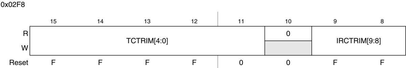
Figure 10-23. S12CPMU IRC1M Trim High Register (CPMUIRCTRIMH)
