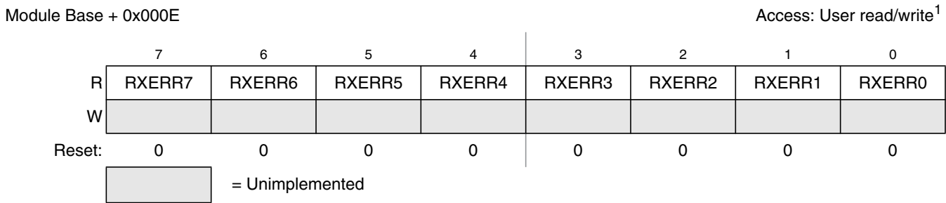
Figure 18-18. MSCAN Receive Error Counter (CANRXERR)
