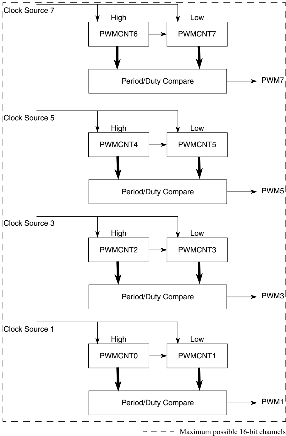
Figure 19-21. PWM 16-Bit Mode
