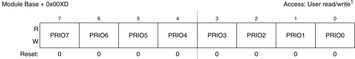
Figure 18-36. Transmit Buffer Priority Register (TBPR)
