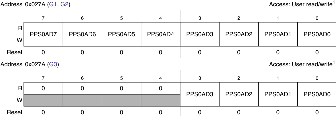
Figure 2-58. Port AD Polarity Select Register (PPS0AD)
