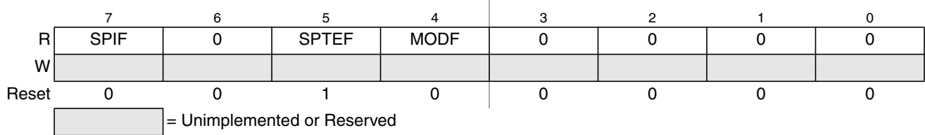
Figure 21-6. SPI Status Register (SPISR)
