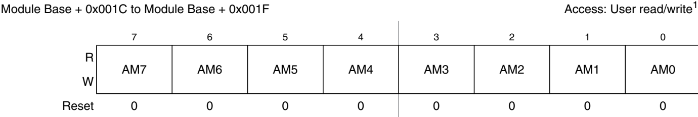
Figure 18-23. MSCAN Identifier Mask Registers (Second Bank) — CANIDMR4–CANIDMR7
