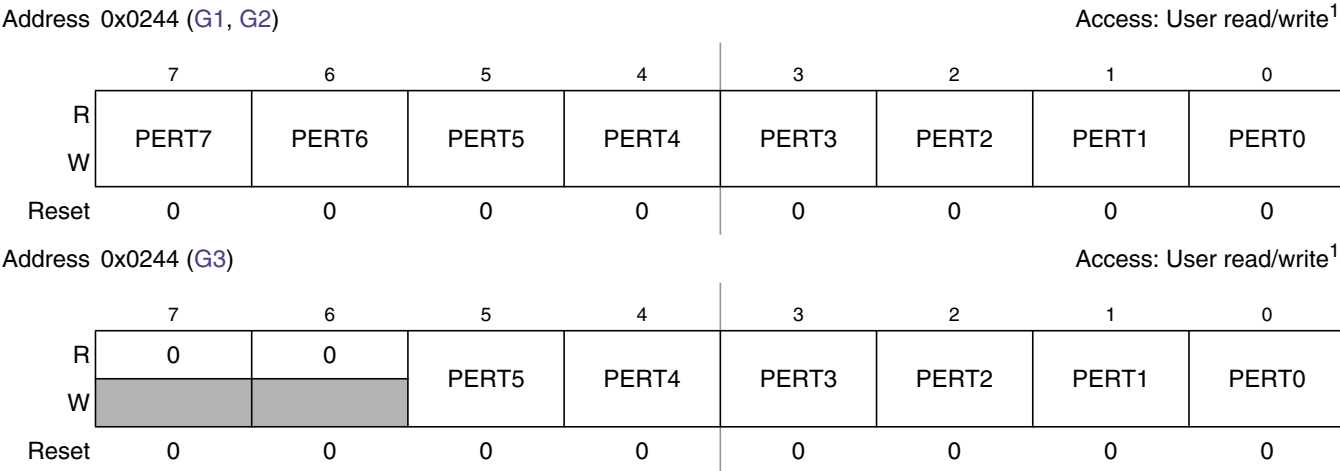
Figure 2-19. Port T Pull Device Enable Register (PERT)
