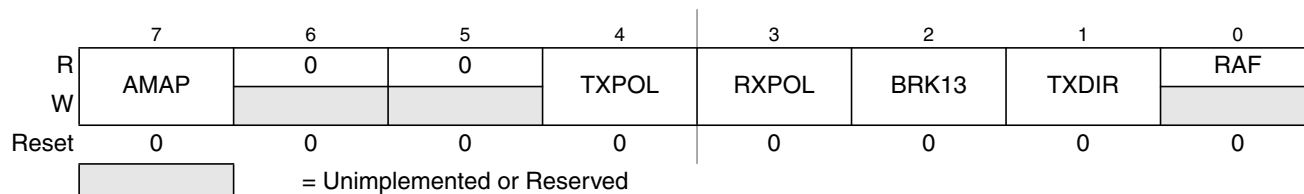
Figure 20-11. SCI Status Register 2 (SCISR2)
