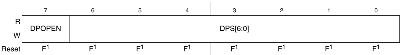
Figure 28-15. EEPROM Protection Register (EEPROT)
