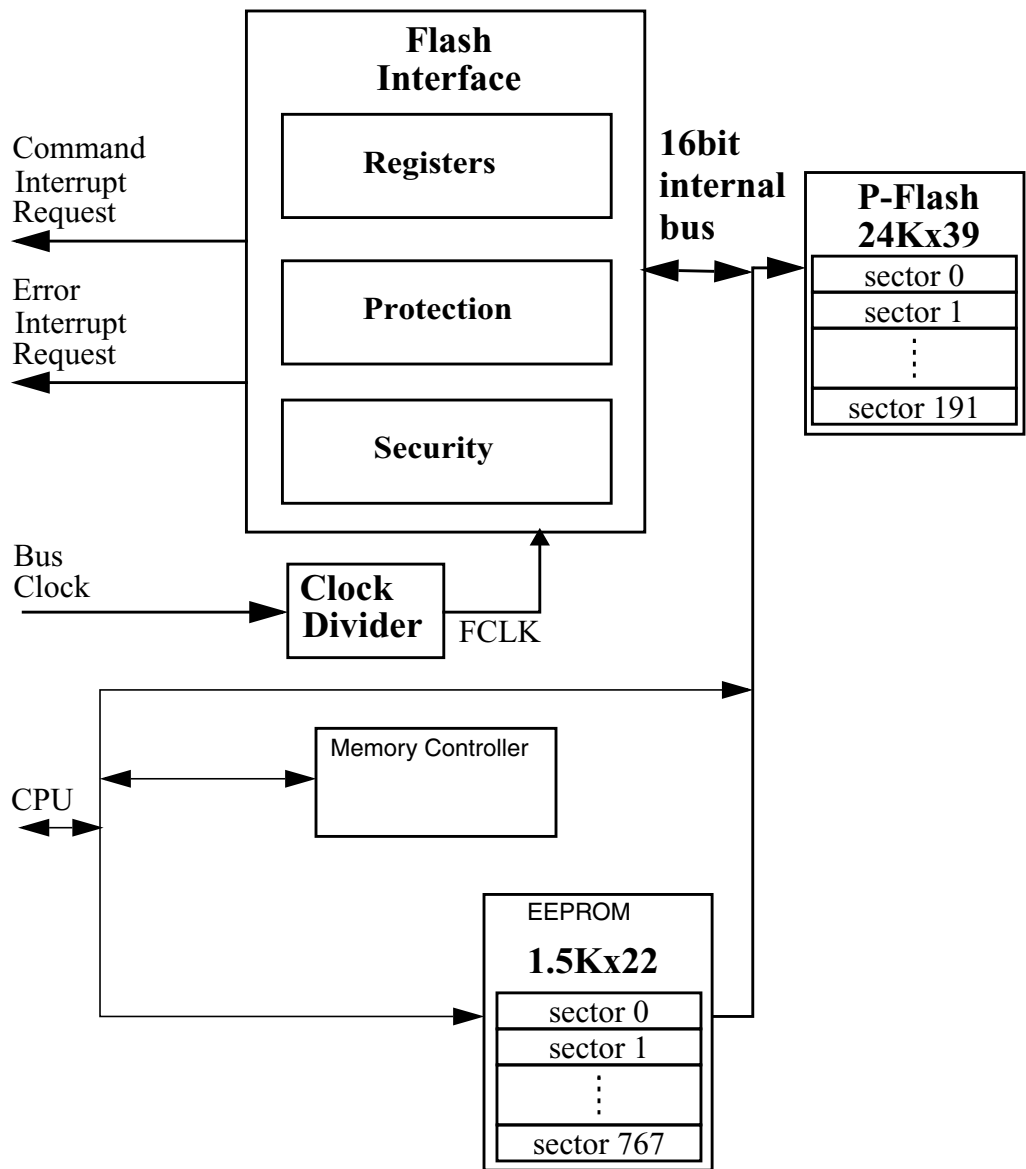
Figure 28-1. FTMRG96K1 Block Diagram
