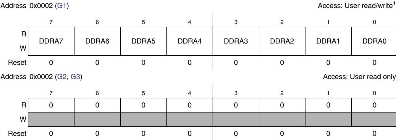
Figure 2-4. Port A Data Direction Register (DDRA)
