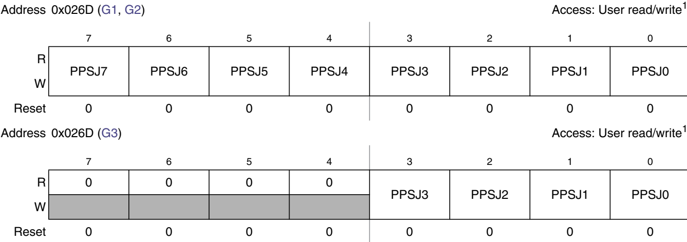
Figure 2-46. Port J Polarity Select Register (PPSJ)
