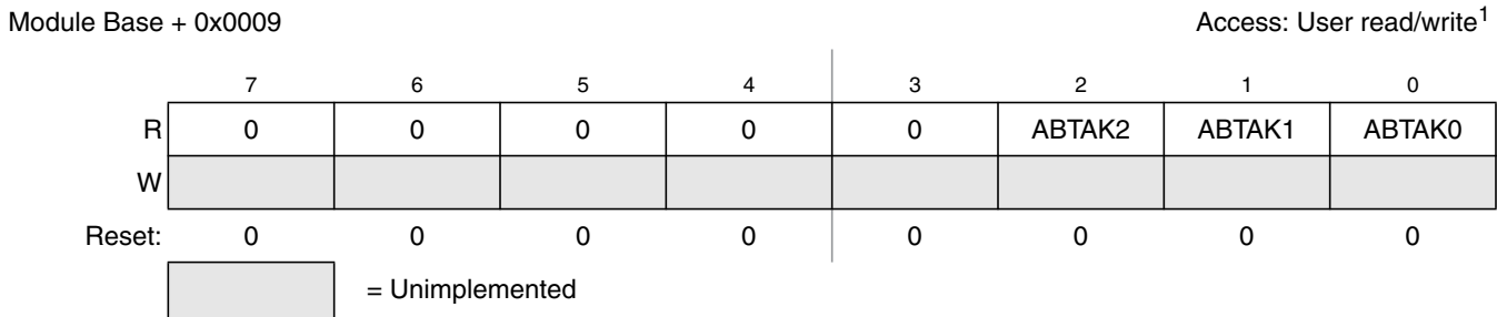
Figure 18-13. MSCAN Transmitter Message Abort Acknowledge Register (CANTAABK)
