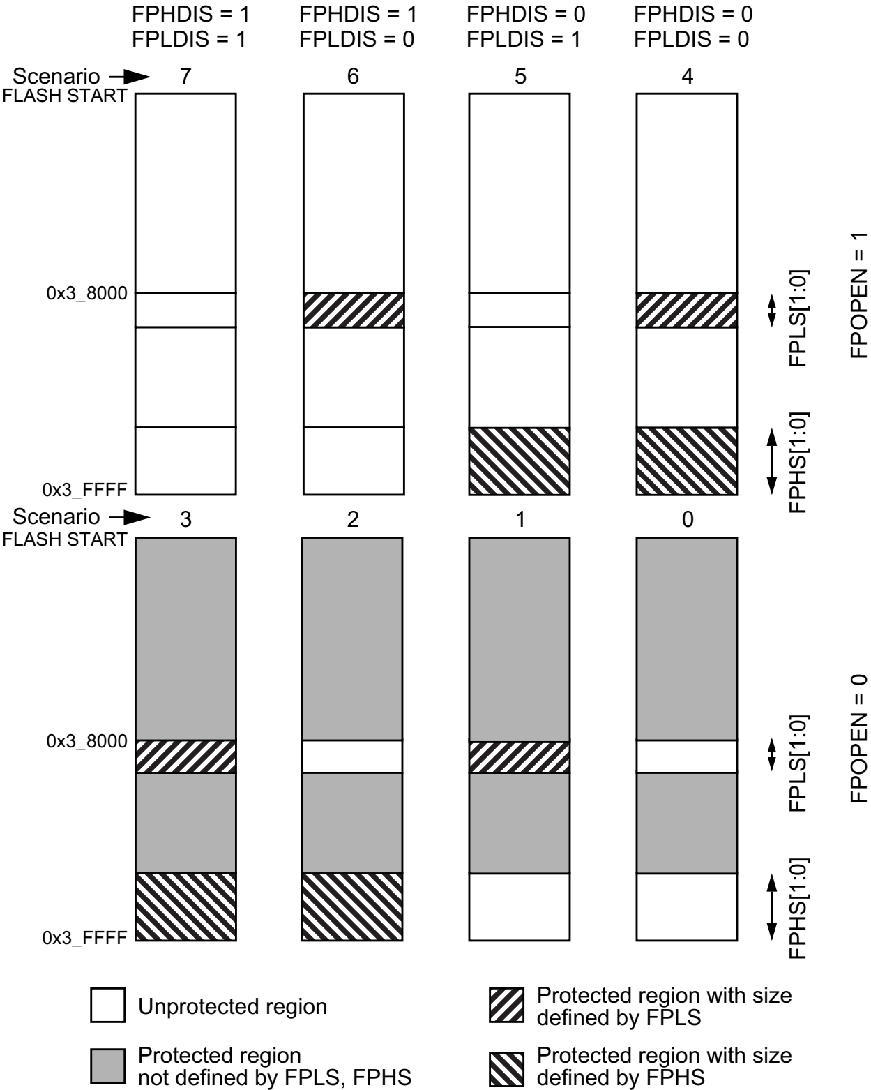
Figure 31-14. P-Flash Protection Scenarios
