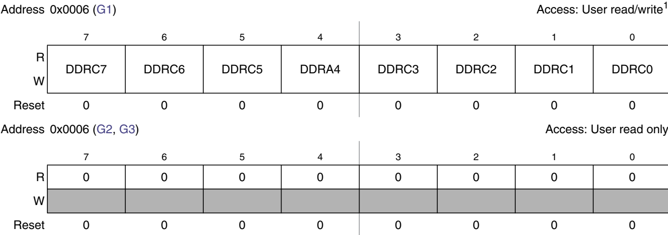
Figure 2-8. Port C Data Direction Register (DDRC)
