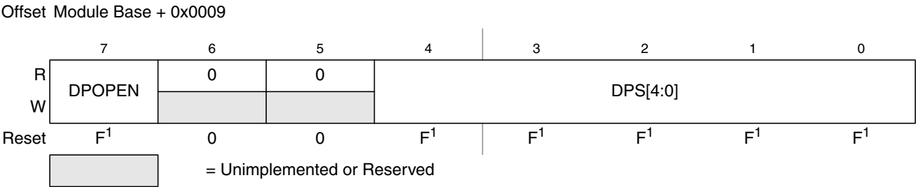
Figure 24-14. EEPROM Protection Register (EEPROT)
