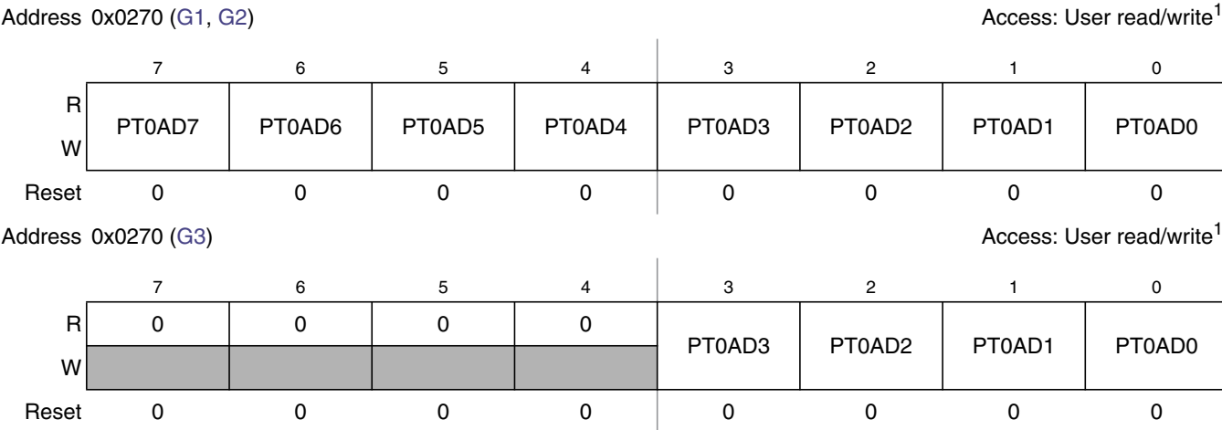
Figure 2-49. Port AD Data Register (PT0AD)
