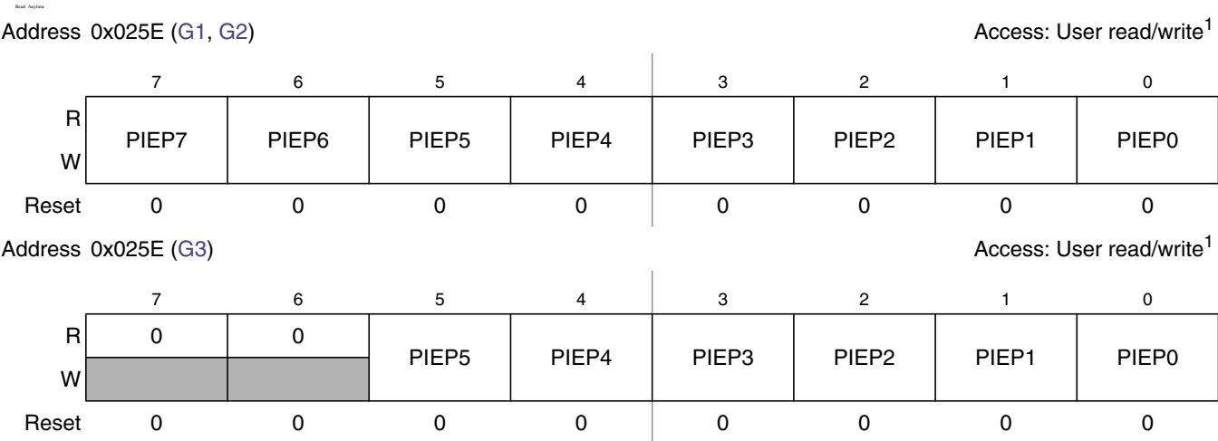
Figure 2-40. Port P Interrupt Enable Register (PIEP)
