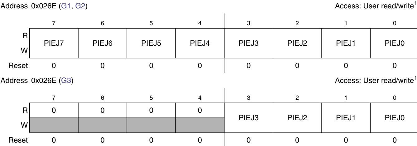
Figure 2-47. Port J Interrupt Enable Register (PIEJ)
