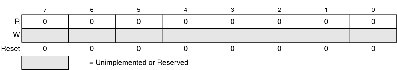
Figure 31-25. Flash Reserved7 Register (FRSV7)
