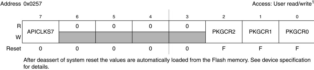
Figure 2-34. Package Code Register (PKGCR)
