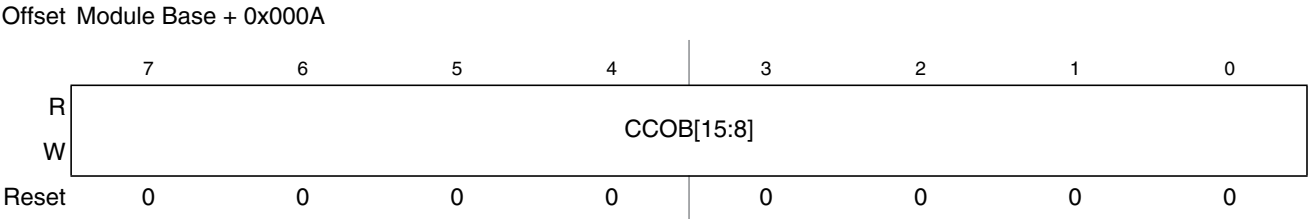
Figure 30-16. Flash Common Command Object High Register (FCCOBHI)
