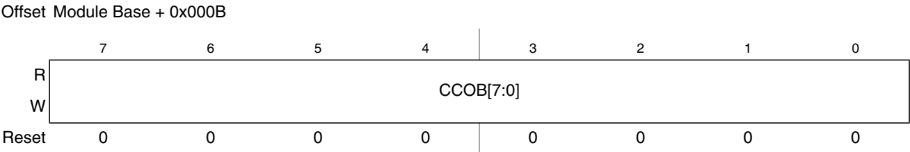
Figure 30-17. Flash Common Command Object Low Register (FCCOBLO)
