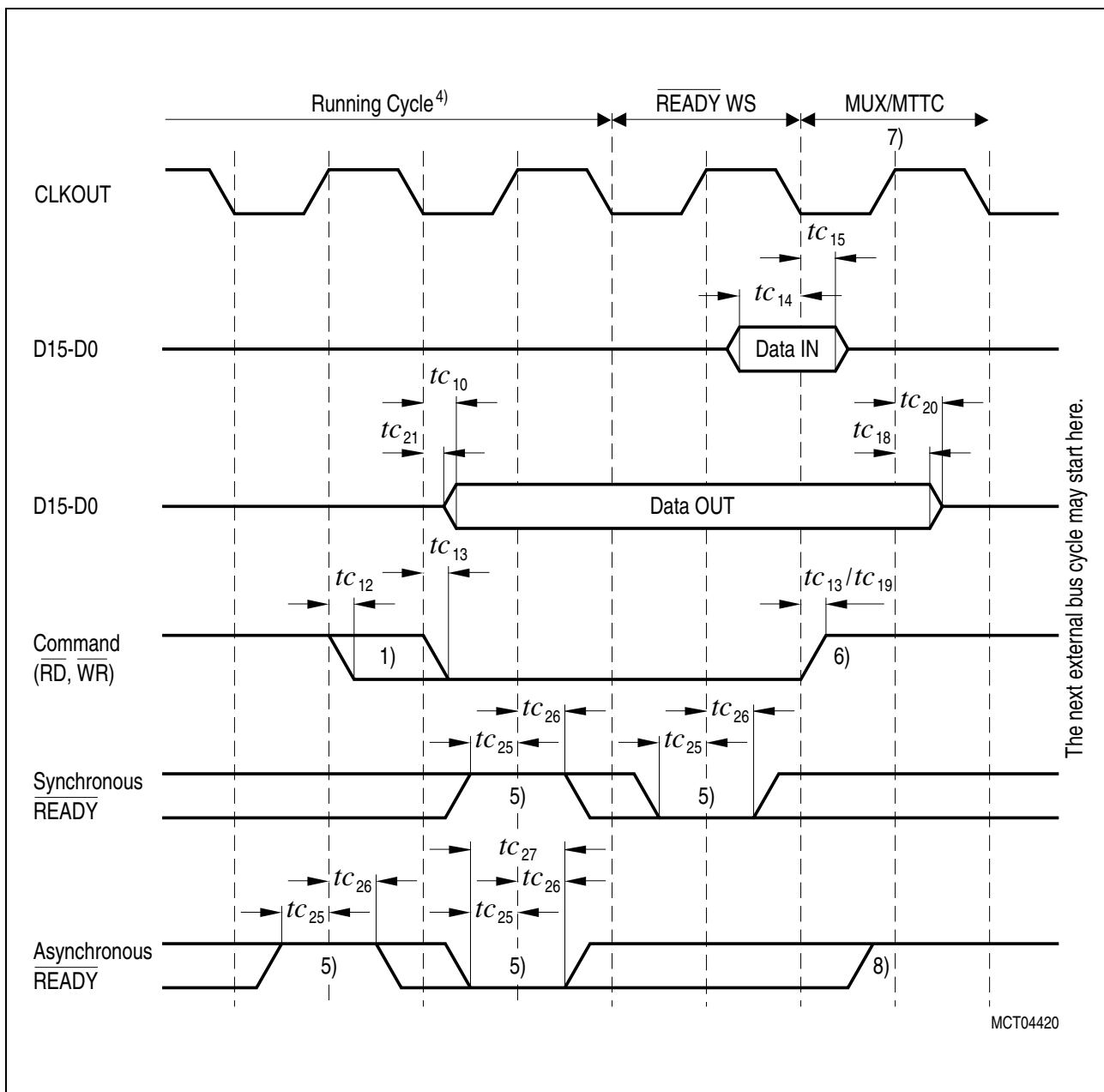
Figure 20 \overline{\text{READY}} Timings
