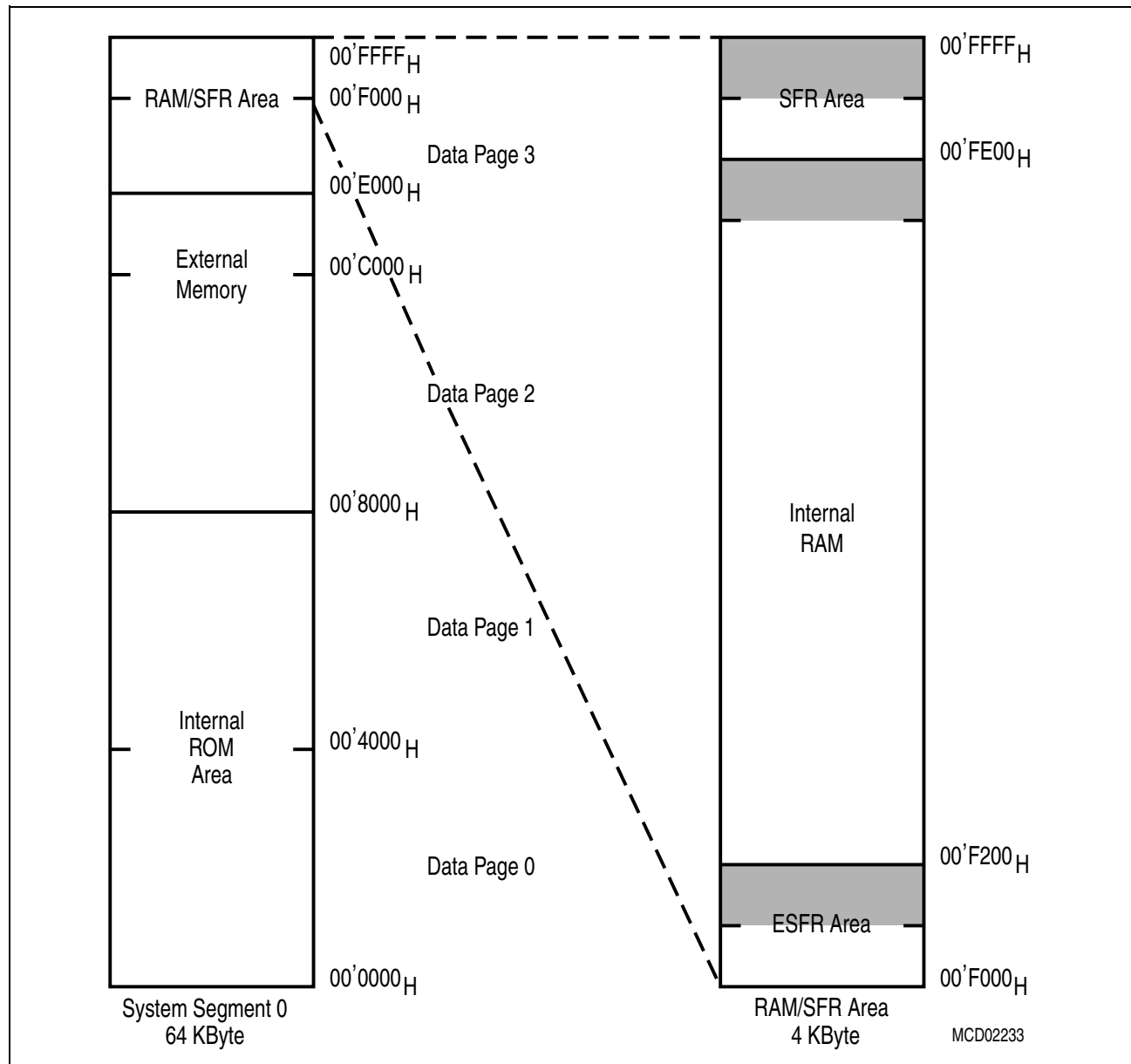
Figure 10 Internal RAM Area and SFR Areas
