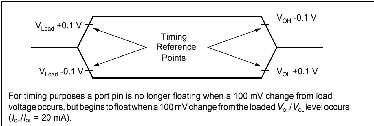
Figure 125 Float Waveforms
