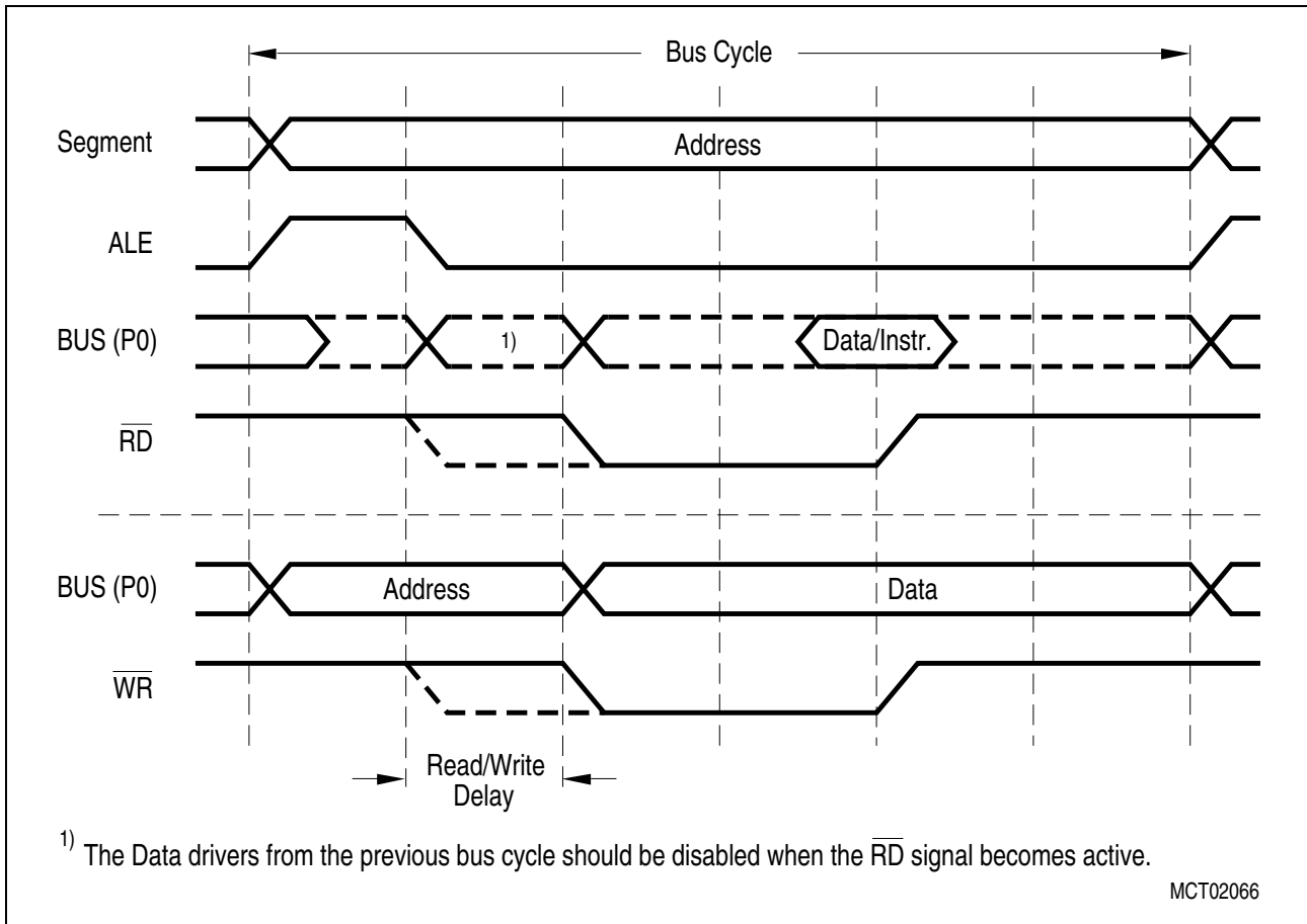
Figure 51 Read/Write Delay
