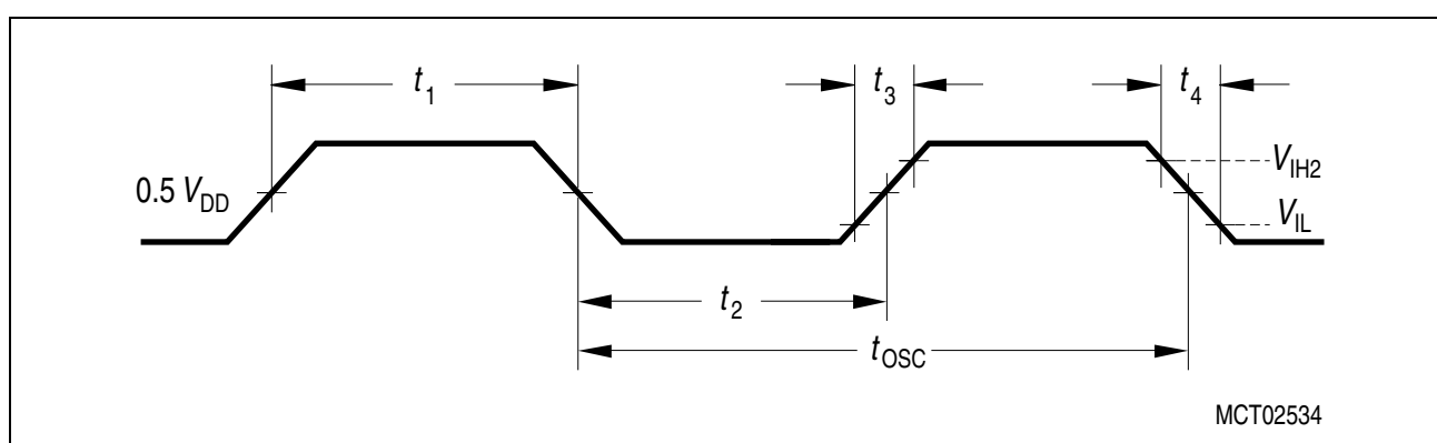
Figure 128 External Clock Drive XTAL1
