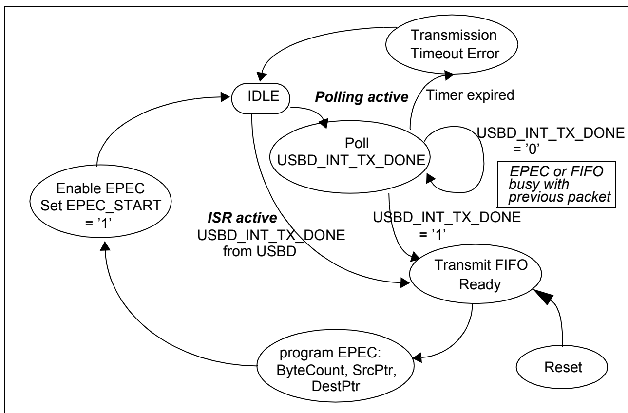
Figure 103 USB IN-Transfer controlled by SW
