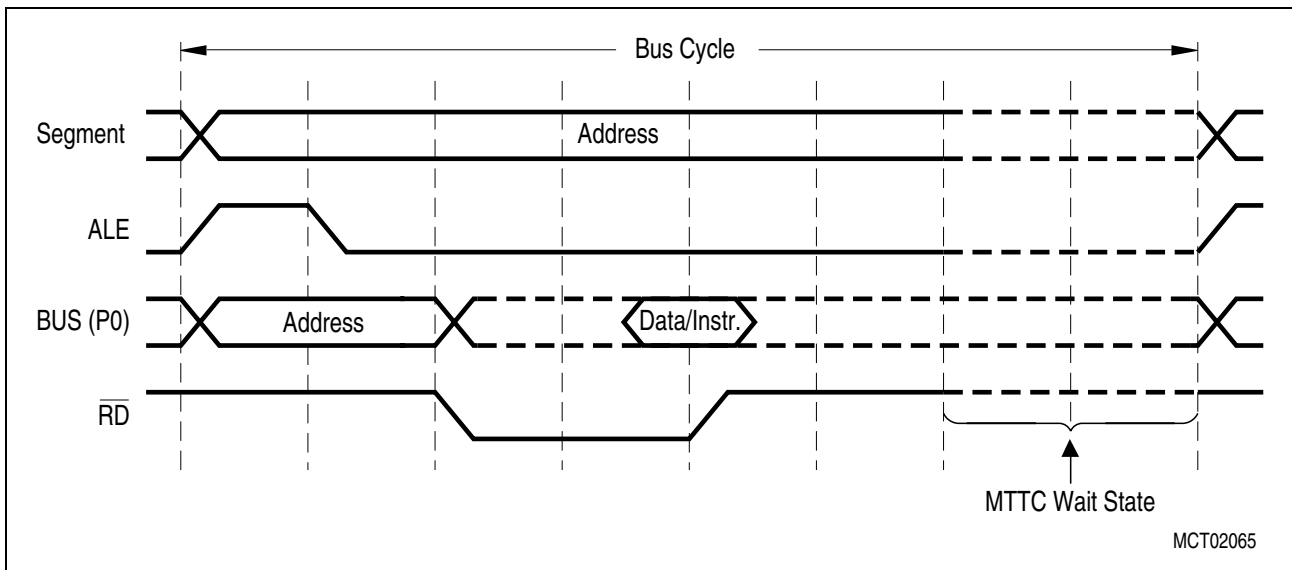
Figure 50 Memory Tri-State Time
