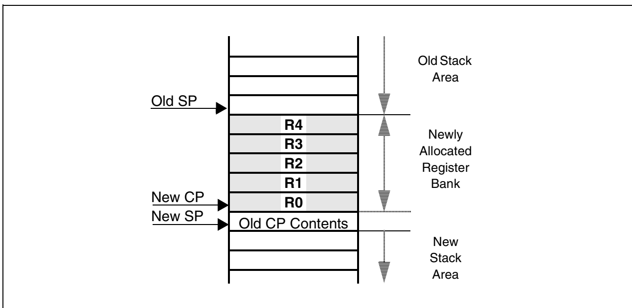
Figure 123 Local Registers
