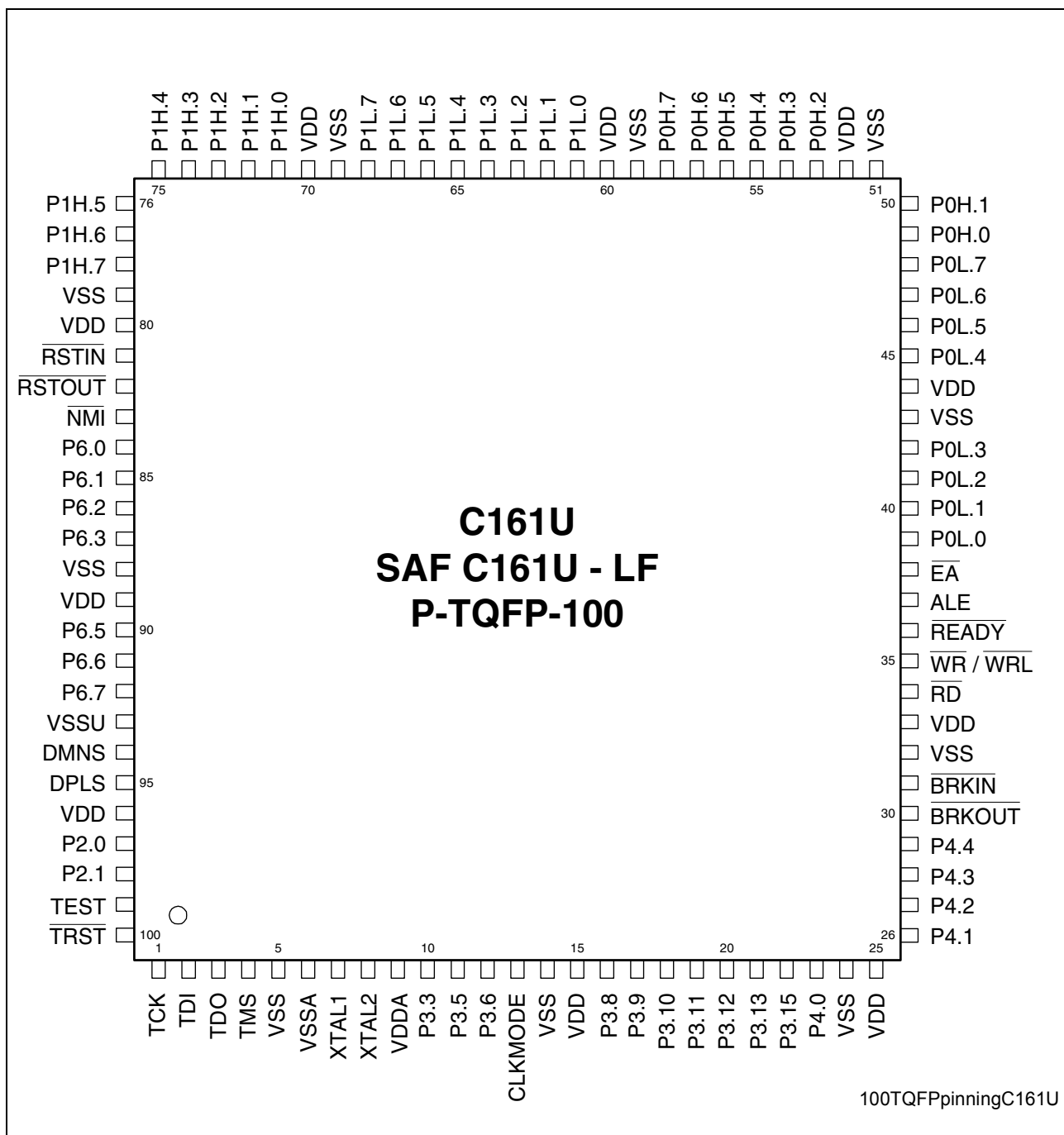
Figure 2 Pinning Diagram of the C161U
