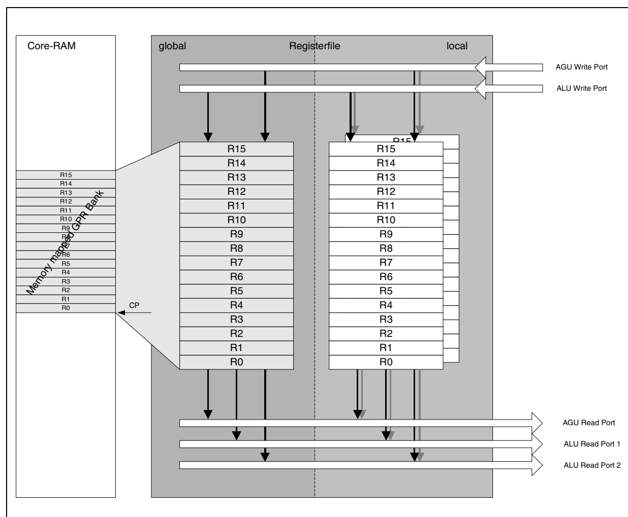
Figure 2-8 Register File
