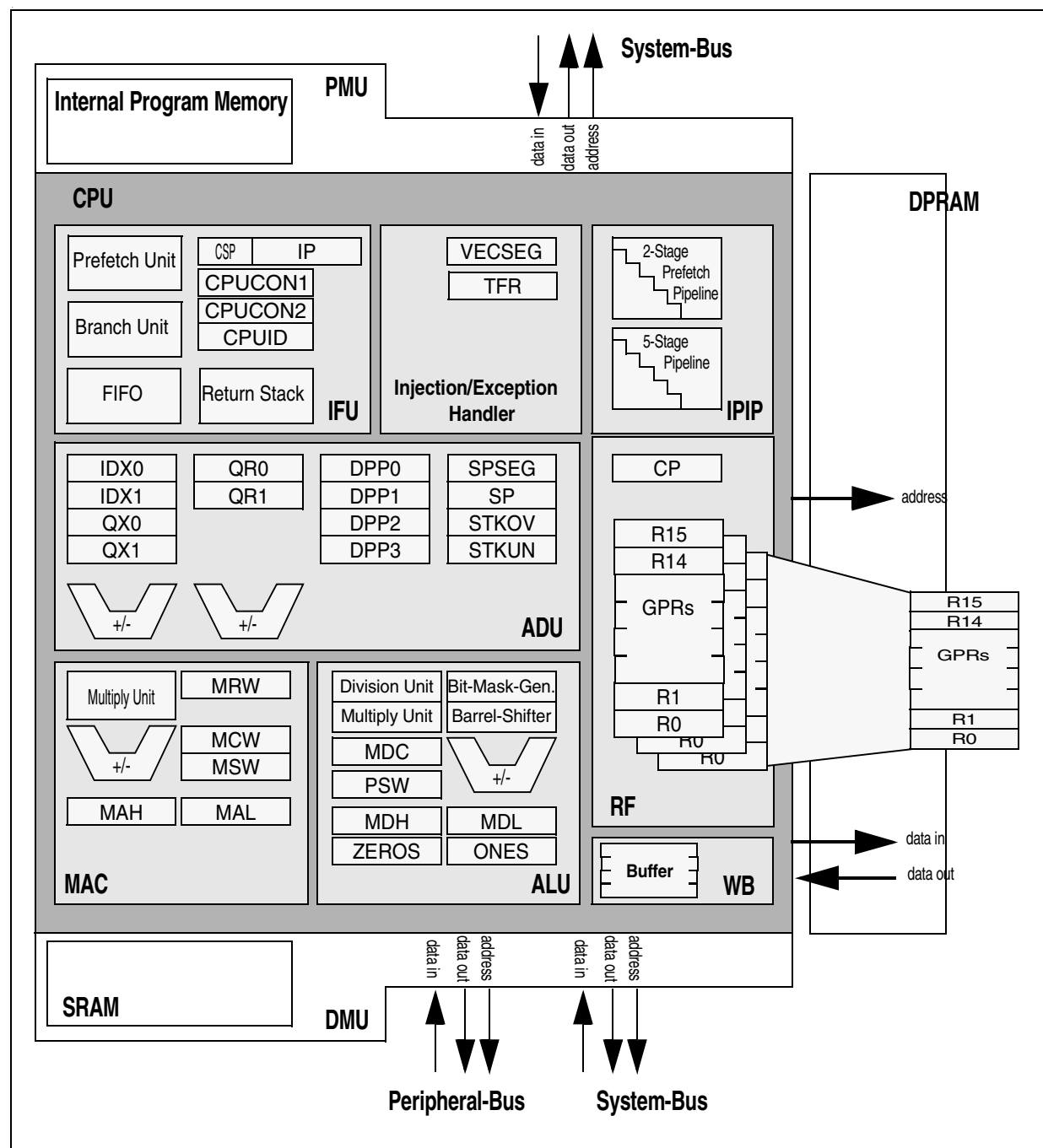
Figure 2-1 CPU Architecture
