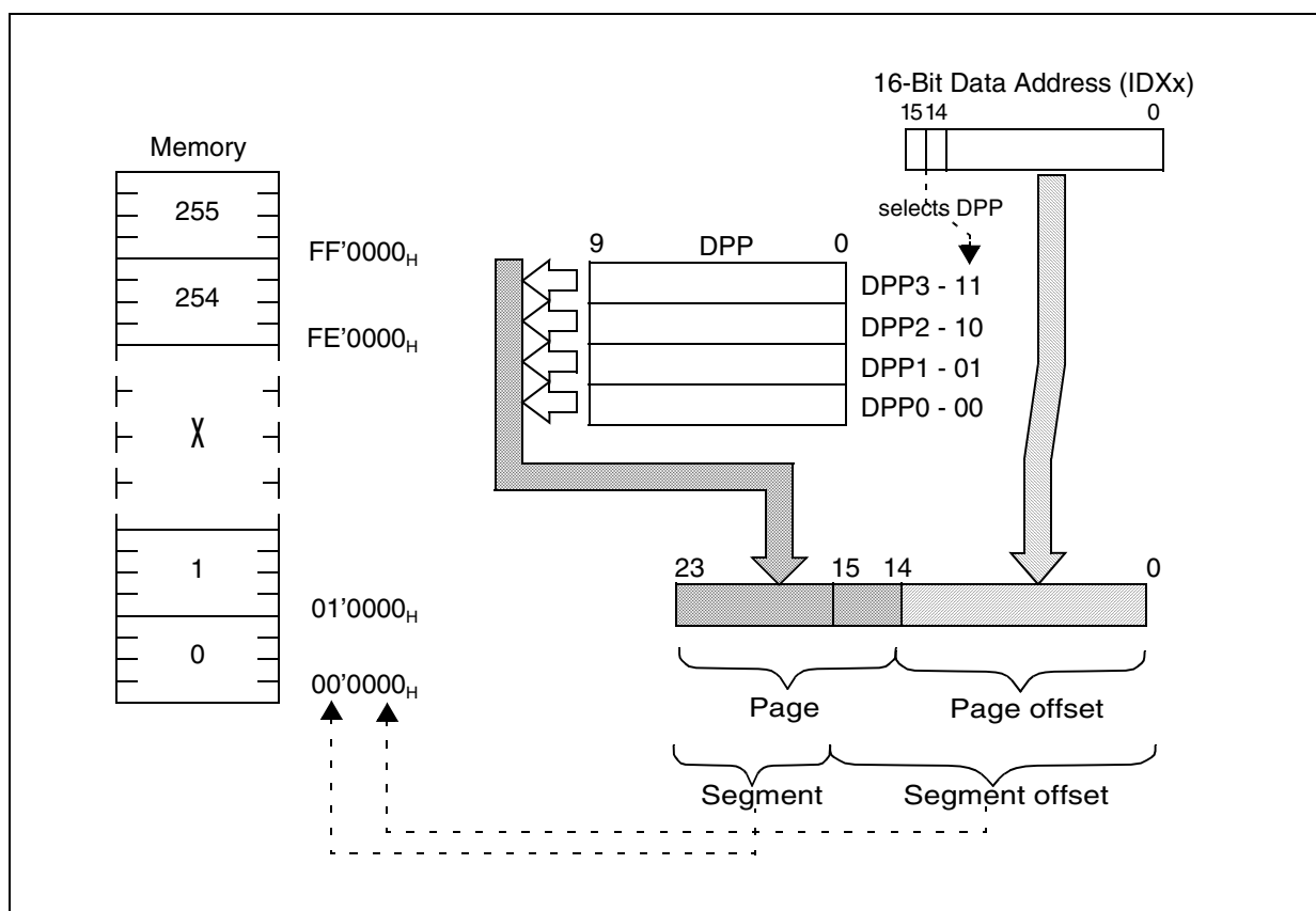
Figure 2-18 CoMOV Operations and Addressing via the IDX Pointers
