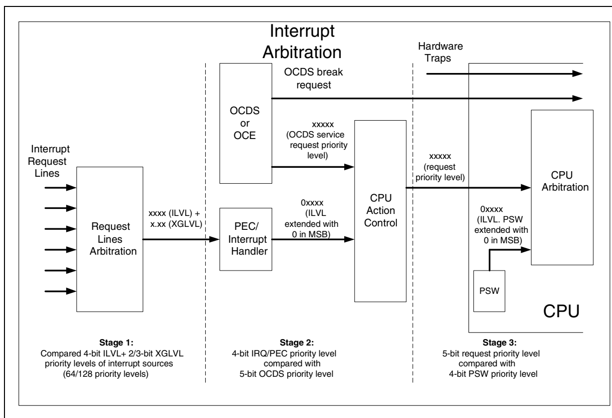
Figure 5-2 Interrupt Arbitration
