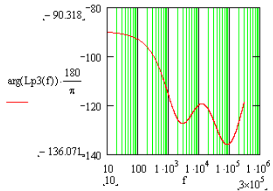
Figure 18. Typical loop transfer function Bode plot of the Boost converter.
