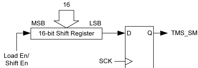
Figure 3. TMS_SM Shifter
