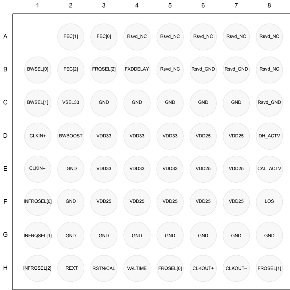
Top View
