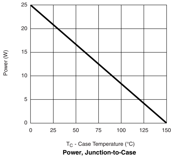
Power, Junction-to-Case
