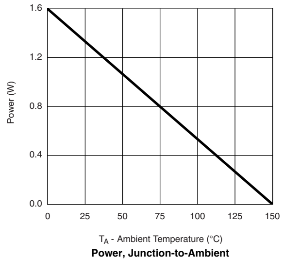
Power, Junction-to-Ambient
