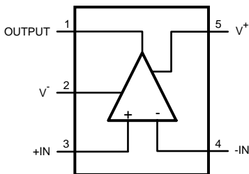
Figure 3. 5-Pin SOT-23, Top View See DBV Package
