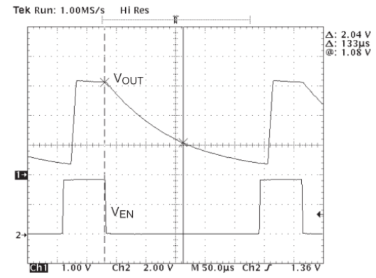
Fig. 7: Turn-Off Time, R_{LOAD}=30K\Omega (0.1mA)
