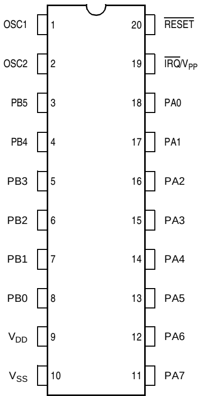
Figure 1-2. Pin Assignments
