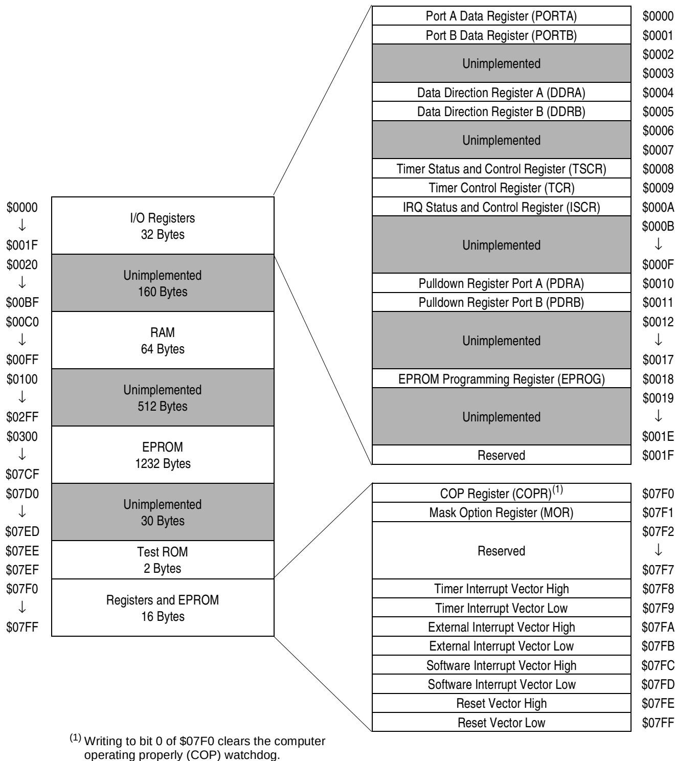
Figure 2-1. Memory Map
