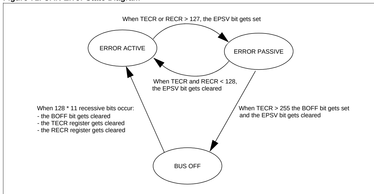
Figure 71. CAN Error State Diagram
