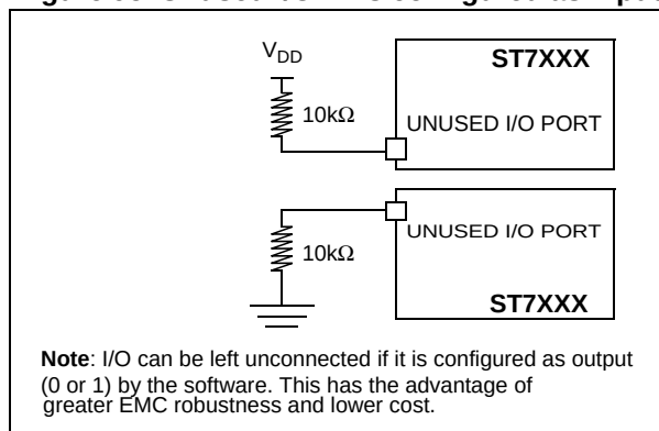
Figure 95. Unused I/O Pins configured as input
