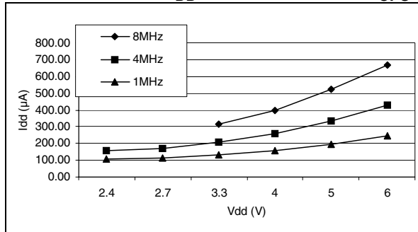
Figure 80. Typical I_{DD} in SLOW-WAIT vs. f_{CPU}
