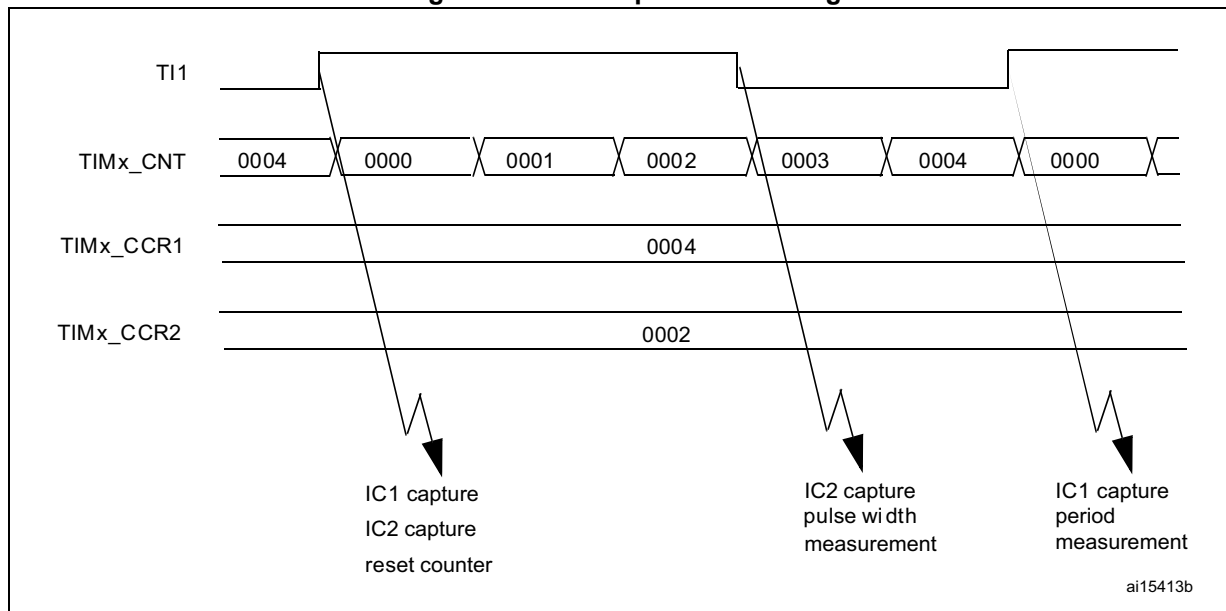
Figure 32. PWM input mode timing
