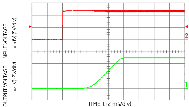
Figure 16. Typical Start-Up with application of V_{in} with low-ESR polymer capacitors at the output ( 7 \times 150\text{ }\mu\text{F} ) ( V_{in} = 12\text{ Vdc} , V_o = 5.0\text{ Vdc} , I_o = 10\text{ A} , C_o = 1050\text{ }\mu\text{F} ).
