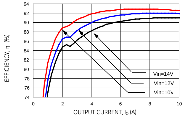
Figure 4. Converter Efficiency versus Output Current ( V_{out} = 2.5Vdc ).
