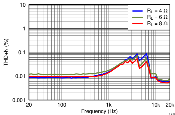
PVDD = 12 V, P_{\text{OSPK}} = 1 \text{ W} Figure 35. THD+N vs Frequency
