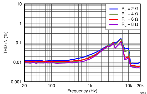
PVDD = 24 V, P_{\text{OSPK}} = 1 \text{ W} Figure 36. THD+N vs Frequency
