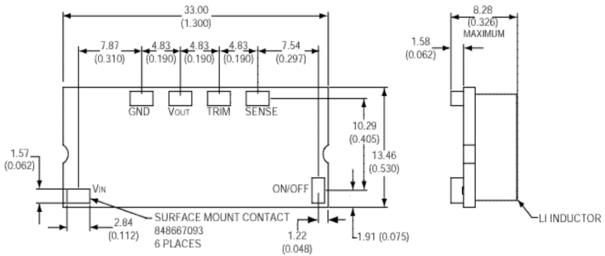
BOTTOM VIEW OF BOARD
