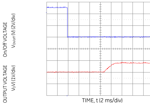
Figure 18. Typical Start-Up Using Remote On/Off with Prebias ( V_{in} = 3.3\text{Vdc} , V_o = 1.8\text{Vdc} , I_o = 1.0\text{A} , V_{bias} = 1.0\text{Vdc} ).
