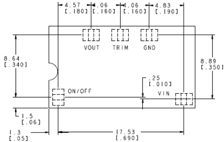
RECOMMENDED PAD LAYOUT PAD SIZE: MIN: 0.120" X 0.095" MAX: 0.135" X 0.110" ALL DIMENSIONS ARE IN MM and [INCHES]
