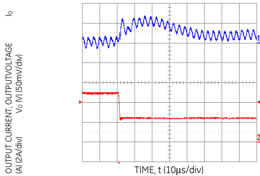
Figure 14. Transient Response to Dynamic Load Change from 100% of 50% full load ( V_o = 5.0\text{Vdc} , C_{ext} = 2 \times 150\ \mu\text{F} Polymer Capacitors).
