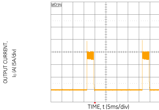
Figure 19. Output short circuit Current ( V_{in} = 5.0\text{Vdc} , V_o = 0.75\text{Vdc} ).
