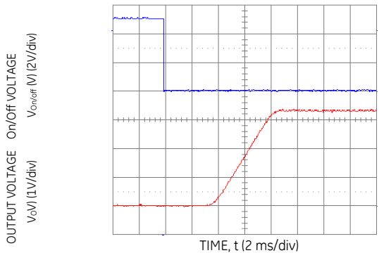
Figure 16. Typical Start-Up Using Remote On/Off with Low-ESR external capacitors ( 7 \times 150\ \mu\text{F} Polymer) ( V_{in} = 5.0\text{Vdc} , V_o = 3.3\text{Vdc} , I_o = 5.0\text{A} , C_o = 1050\ \mu\text{F} ).
