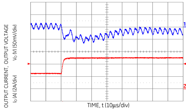
Figure 13. Transient Response to Dynamic Load Change from 50% to 100% of full load (Vo = 5.0 Vdc, Cext = 2x150 μF Polymer Capacitors).
