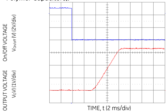
Figure 15. Typical Start-Up Using Remote On/Off ( V_{in} = 5.0\text{Vdc} , V_o = 3.3\text{Vdc} , I_o = 5.0\text{A} ).
