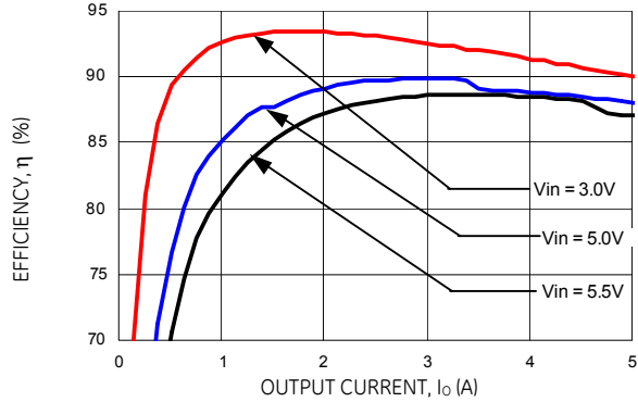
Figure 4. Converter Efficiency versus Output Current (Vout = 1.8Vdc).
