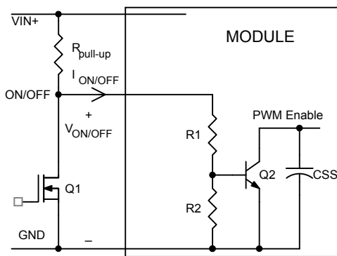
Figure 30. Remote On/Off Implementation using logic-level devices and an external pull-up resistor.
