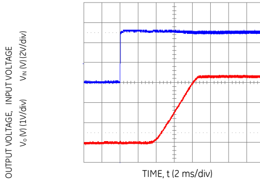
Figure 17. Typical Start-Up with application of V_{in} ( V_{in} = 5.0\text{Vdc} , V_o = 3.3\text{Vdc} , I_o = 5\text{A} ).
