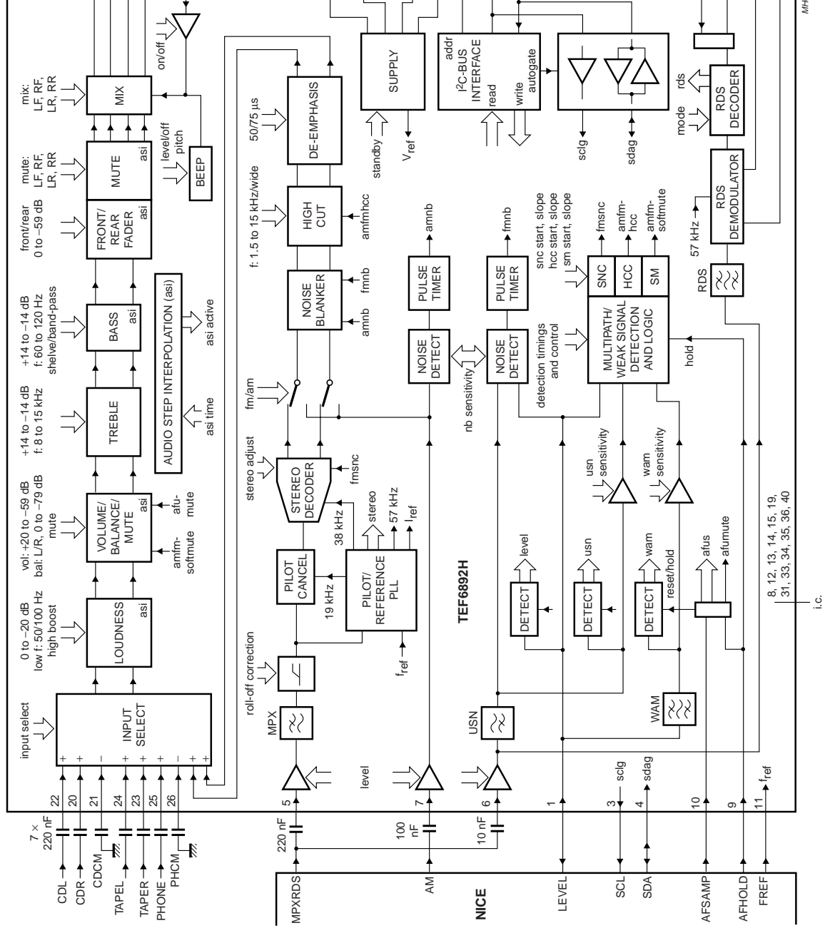
Fig.24 Application diagram.
