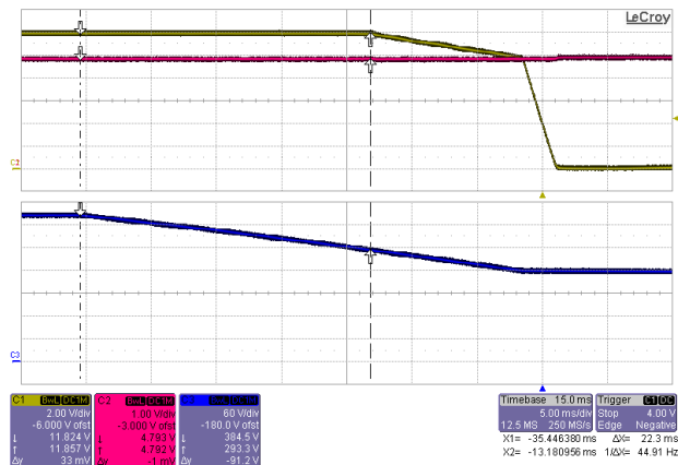
Figure 34 – Maximum Hold-Up Time = 22.3 ms Upper (Yellow): V_{MAIN} , 2 V / div. Upper (Red): V_{STBY} , 1 V / div. Lower: Input VDC, 60 V, 5 ms / div.
