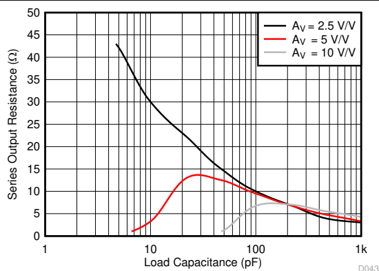
Figure 6-43. Series Output Resistance vs Load Capacitance
