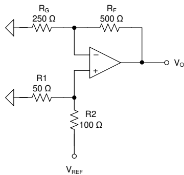
Figure 8-4. Gain Transfer Function from VREF to VO1
