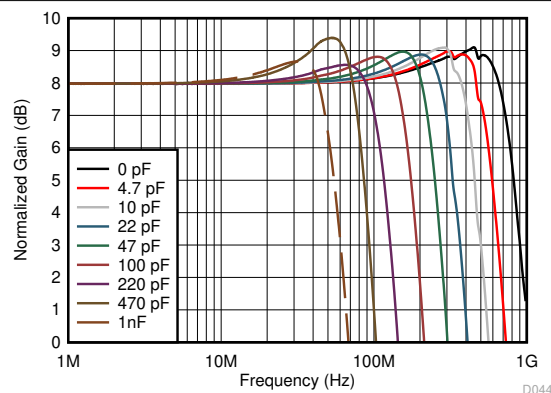
Figure 6-44. Frequency Response vs Load Capacitance
