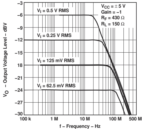
Figure 5-68. Output Amplitude vs Frequency
