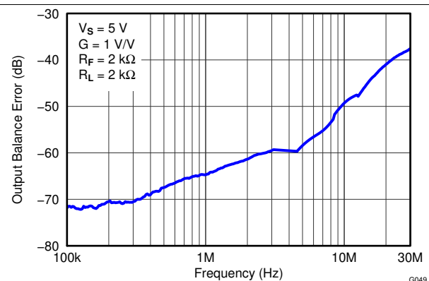
Figure 58. Output Balance Error vs Frequency
