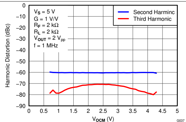
Figure 46. Harmonic Distortion vs V_{OCM} at 1 MHz
