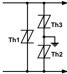
Figure 16. MULTI-POINT PROTECTION
