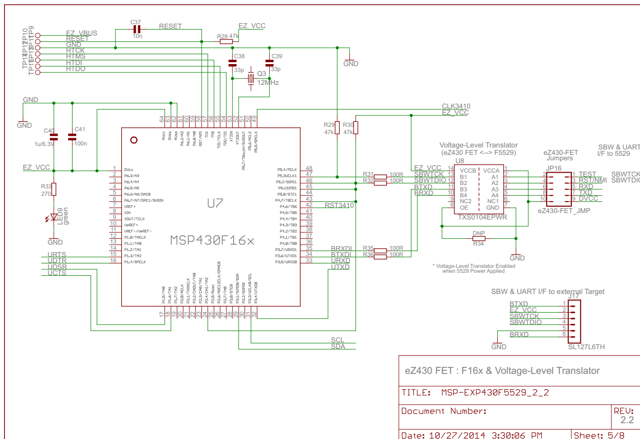
Figure 14. Schematics (5 of 8)
