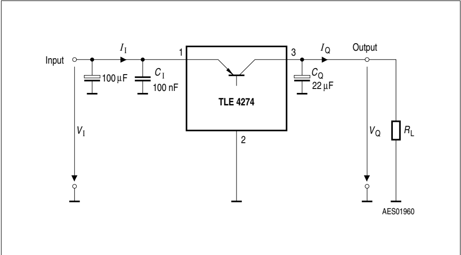
Figure 3 Measuring Circuit
