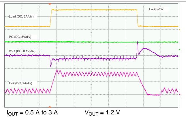
Figure 18. Load Transient
