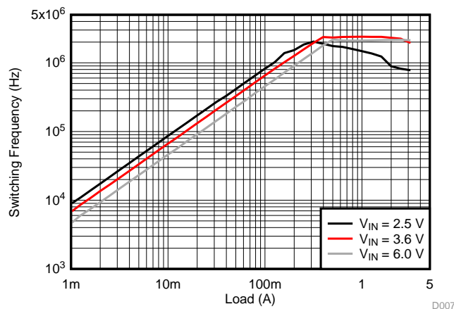
Figure 1. Switching Frequency
