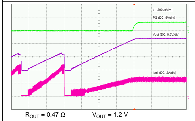
Figure 21. Output Short-Circuit Protection, Recovery
