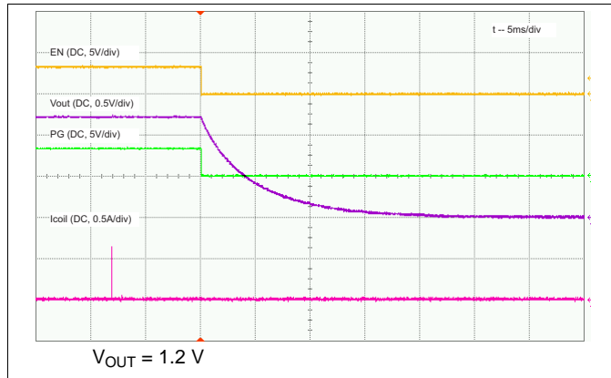
Figure 17. Shutdown without Load
