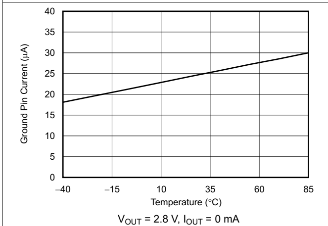
Figure 6-21. Ground Pin Current vs Temperature
