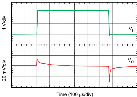
Time (100 \mu\text{s}/\text{div} ) V_{OUT} = 2.8\text{ V} , I_{OUT} = 200\text{ mA} Figure 6-53. Line Transient Response
