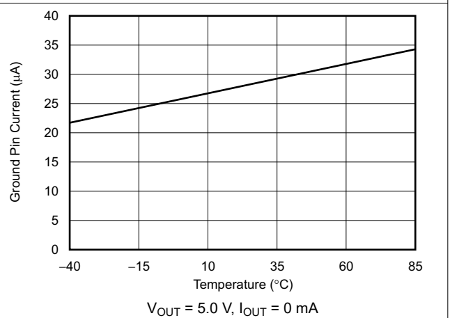
Figure 6-22. Ground Pin Current vs Temperature
