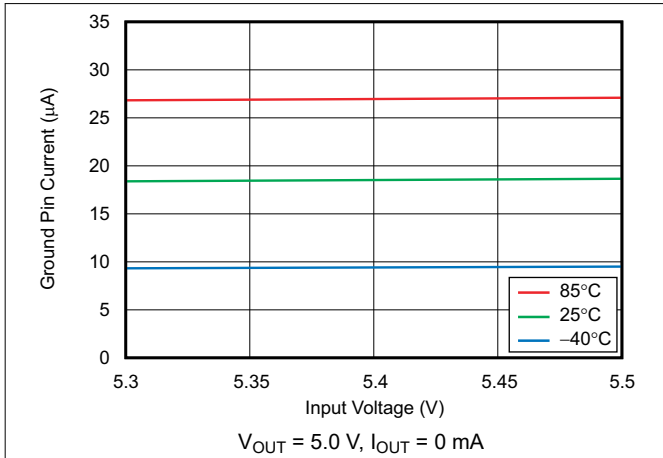
Figure 6-19. Ground Pin Current vs Input Voltage
