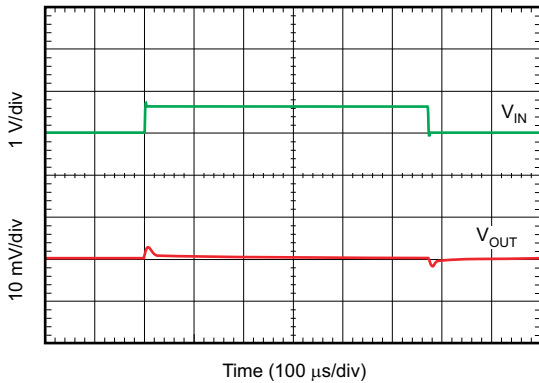
Time (100 \mu\text{s}/\text{div} ) V_{OUT} = 2.8\text{ V} , I_{OUT} = 200\text{ mA} Figure 6-51. Line Transient Response
