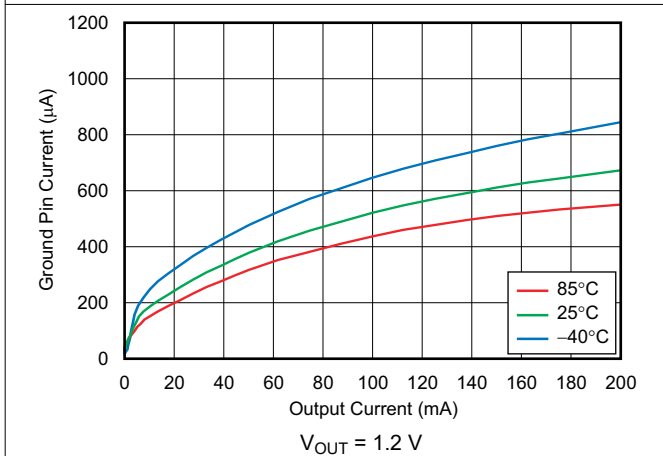
Figure 6-23. Ground Pin Current vs Output Current
