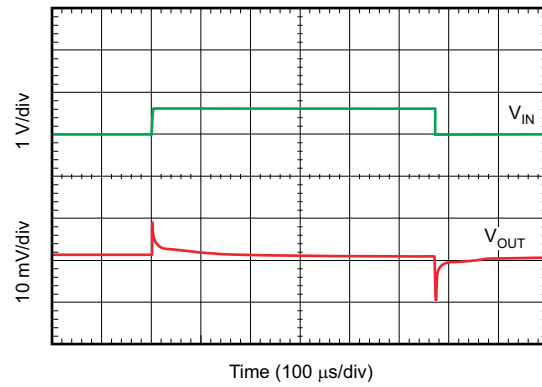
Time (100 \mu\text{s}/\text{div} ) V_{OUT} = 2.8\text{ V} , I_{OUT} = 150\text{ mA} Figure 6-50. Line Transient Response
