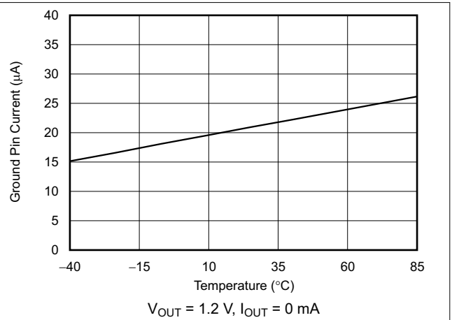
Figure 6-20. Ground Pin Current vs Temperature
