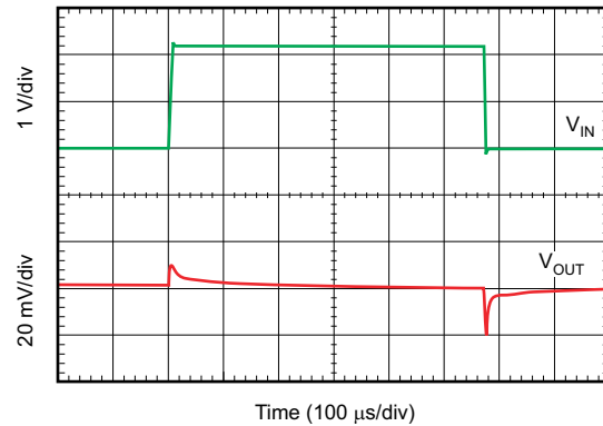
Time (100 \mu\text{s}/\text{div} ) V_{OUT} = 2.8\text{ V} , I_{OUT} = 200\text{ mA} Figure 6-52. Line Transient Response
