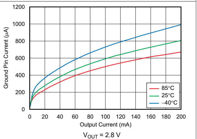
Figure 6-24. Ground Pin Current vs Output Current
