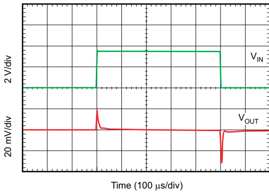
Time (100 \mu\text{s}/\text{div} ) V_{OUT} = 1.2\text{ V} , I_{OUT} = 200\text{ mA} Figure 6-49. Line Transient Response
