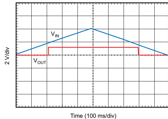
Time (100 \text{ms}/\text{div} ) V_{OUT} = 1.2\text{ V} , I_{OUT} = 30\text{ mA} Figure 6-54. V_{IN} Ramp Up, Ramp Down Response
