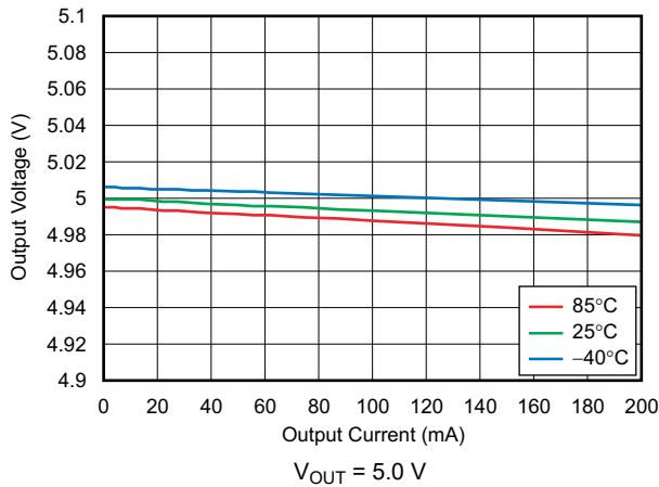
Figure 6-3. Load Regulation
