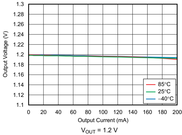
Figure 6-1. Load Regulation
