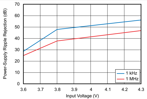
Figure 6-38. Power-Supply Ripple Rejection vs Input Voltage
