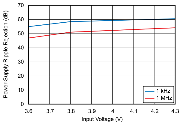
Figure 6-37. Power-Supply Ripple Rejection vs Input Voltage
