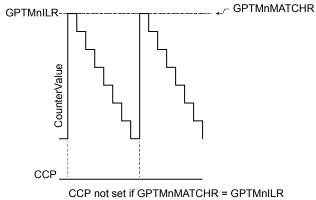
Figure 11-7. CCP Output, GPTMTnMATCHHR = GPTMTnILR
