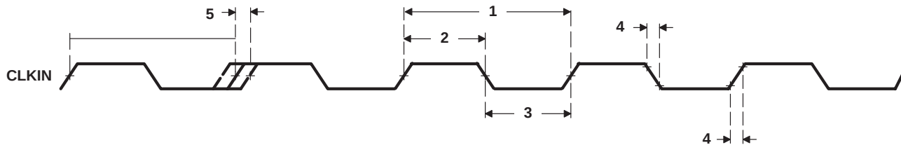
Figure 7–1. CLKIN Timing
