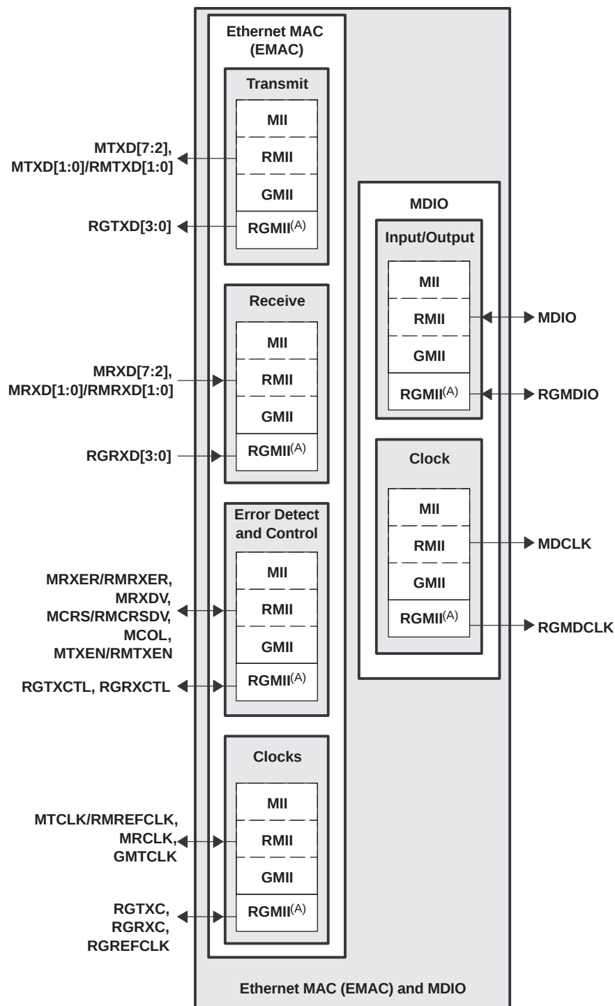
A. RGMII signals are mutually exclusive to all other EMAC signals. Figure 2-10. EMAC/MDIO [MII, GMII, RMII, and RGMII] Peripheral Signals
