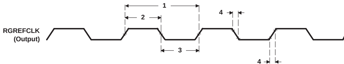
Figure 7-68. RREFCLK Timing
