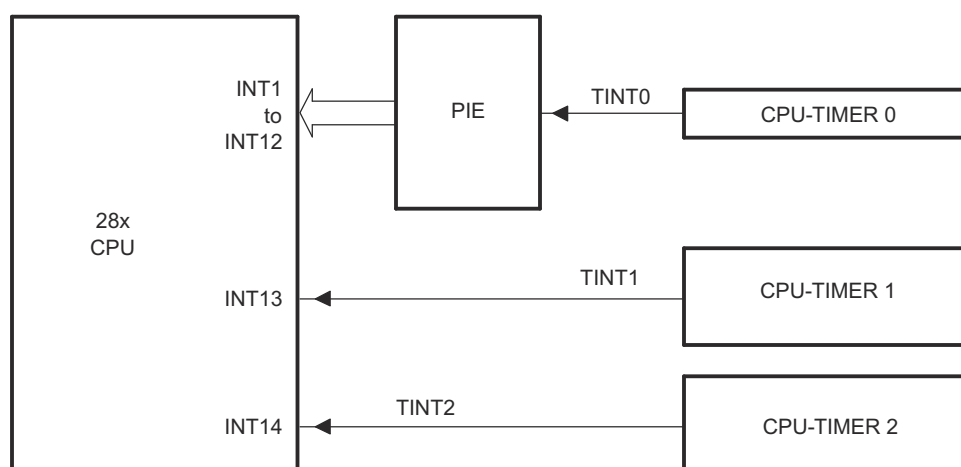
Figure 1-49. CPU-Timers
