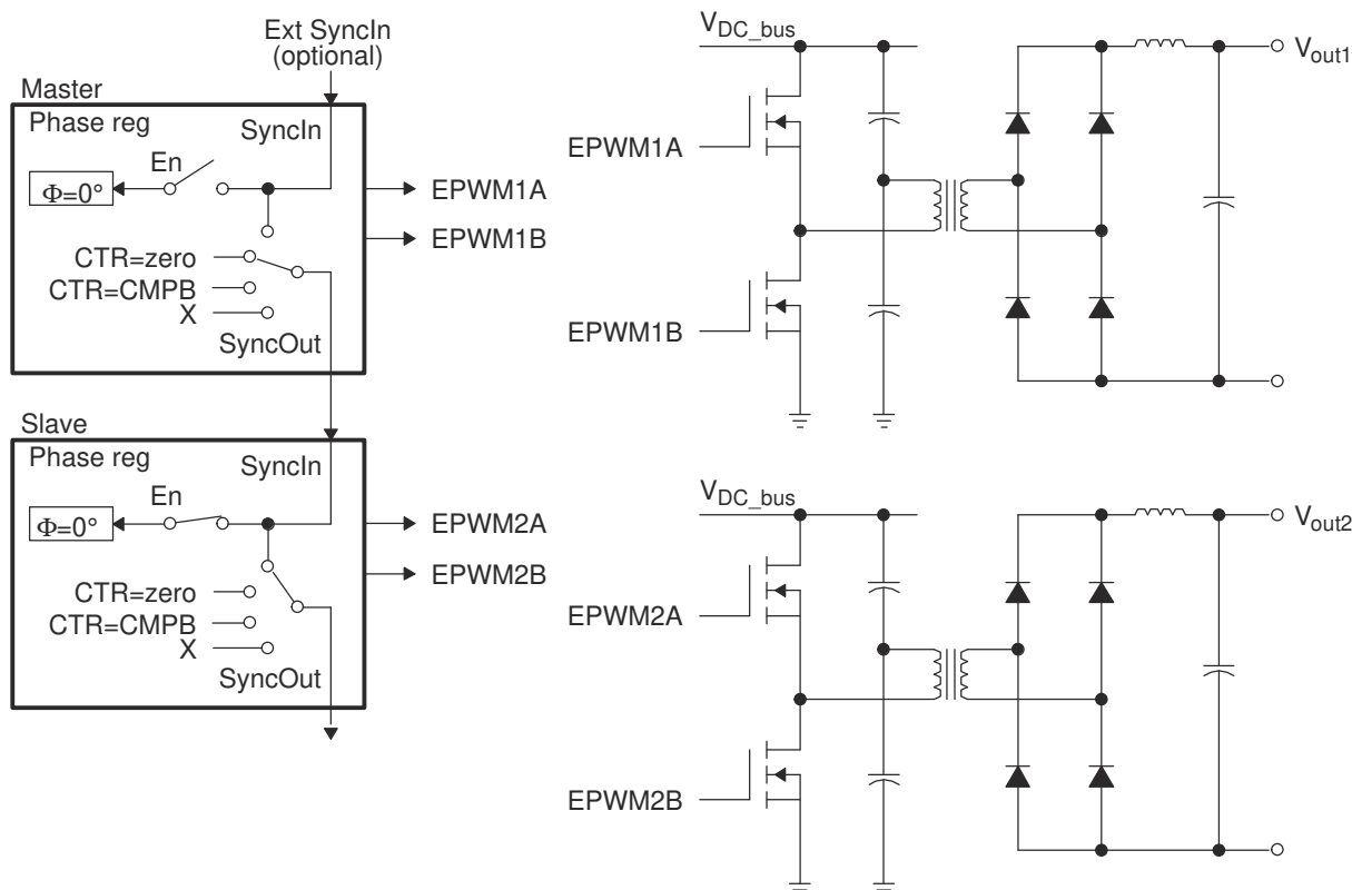
Figure 3-58. Control of Two Half-H Bridge Stages ( F_{P\text{WM}2} = N \times F_{P\text{WM}1} )
