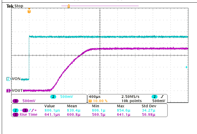
Figure 28. Turn-On Response Time ( V_{IN} = 1.8\text{ V} , C_{IN} = 1\ \mu\text{F} , C_{OUT} = 0.1\ \mu\text{F} , R_{OUT} = 10\ \Omega )
