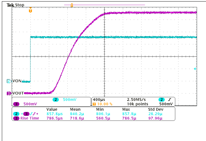
Figure 24. Turn-On Response Time ( V_{IN} = 3.3\text{ V} , C_{IN} = 1\ \mu\text{F} , C_{OUT} = 0.1\ \mu\text{F} , R_{OUT} = 10\ \Omega )
