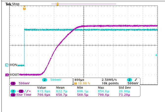
Figure 26. Turn-On Response Time ( V_{IN} = 2.5\text{ V} , C_{IN} = 1\ \mu\text{F} , C_{OUT} = 0.1\ \mu\text{F} , R_{OUT} = 10\ \Omega )
