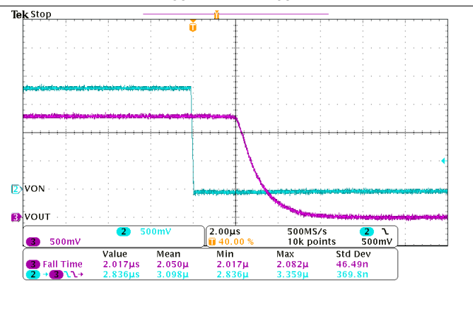
Figure 29. Turn-Off Response Time ( V_{IN} = 1.8\text{ V} , C_{IN} = 1\ \mu\text{F} , C_{OUT} = 0.1\ \mu\text{F} , R_{OUT} = 10\ \Omega )
