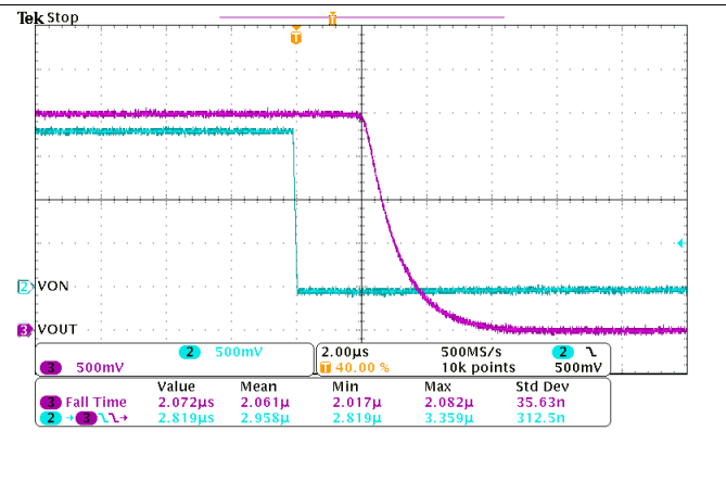
Figure 27. Turn-Off Response Time ( V_{IN} = 2.5\text{ V} , C_{IN} = 1\ \mu\text{F} , C_{OUT} = 0.1\ \mu\text{F} , R_{OUT} = 10\ \Omega )
