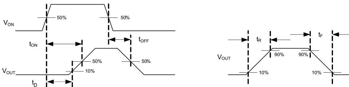
Figure 37. Timing Waveforms
