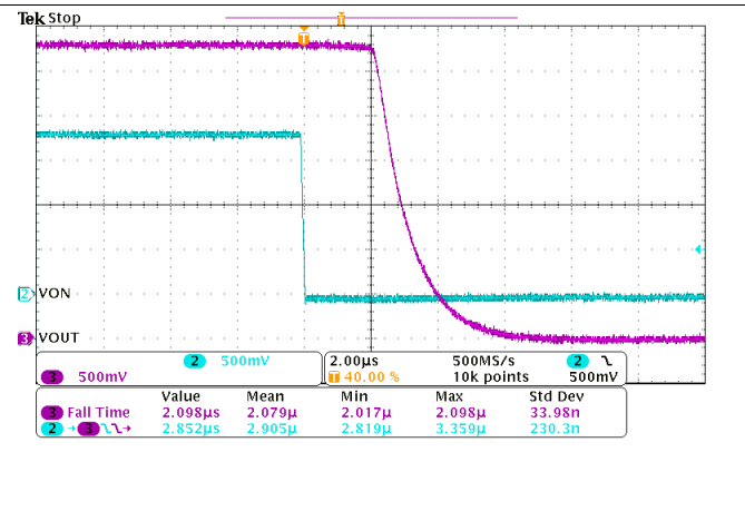
Figure 25. Turn-Off Response Time ( V_{IN} = 3.3\text{ V} , C_{IN} = 1\ \mu\text{F} , C_{OUT} = 0.1\ \mu\text{F} , R_{OUT} = 10\ \Omega )
