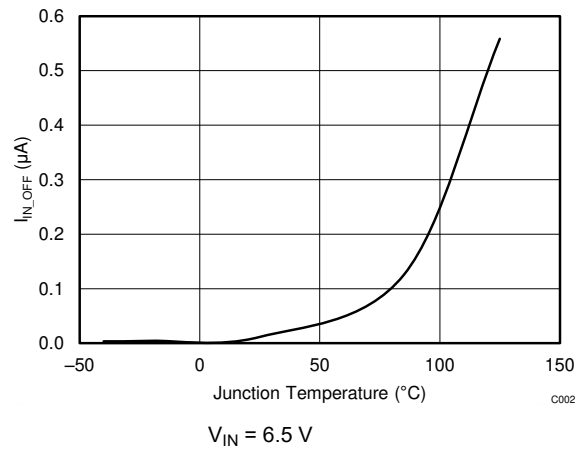
Figure 7-6. Supply Current, Output Disabled ( I_{IN\_OFF} ) vs Temperature
