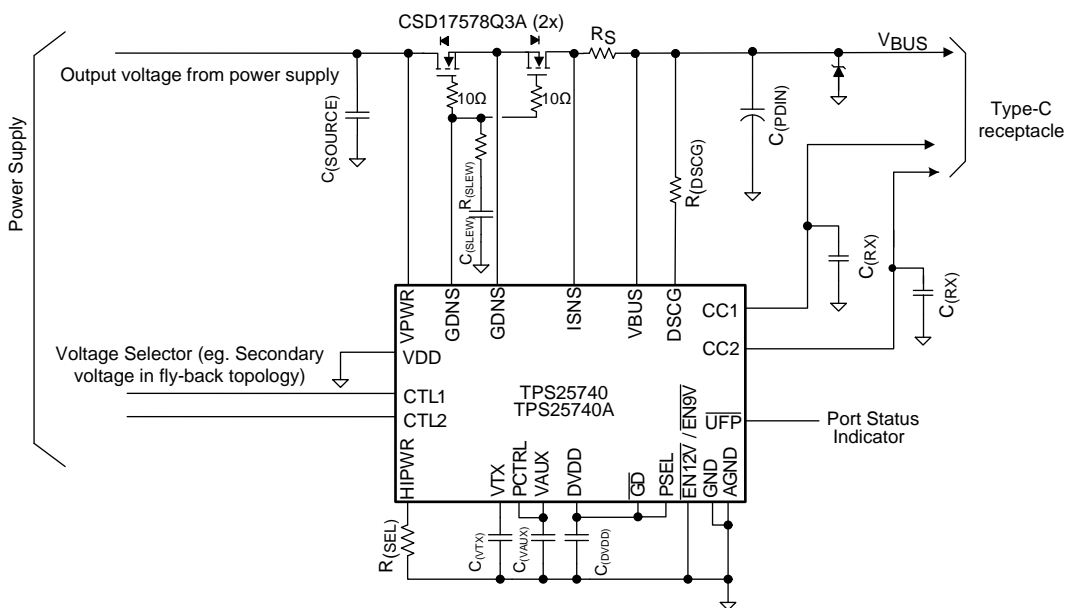
Figure 19. Schematic 1
