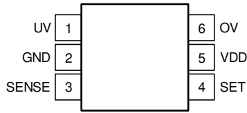
Figure 4-1. DDC Package SOT-6 Top View
