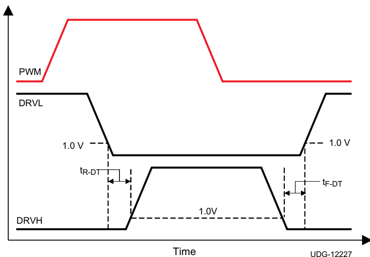
Figure 18. Dead-Time Definitions
