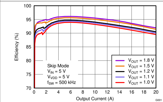
Figure 6-33. Efficiency vs Output Current
