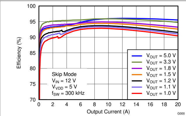
Figure 6-29. Efficiency vs Output Current
