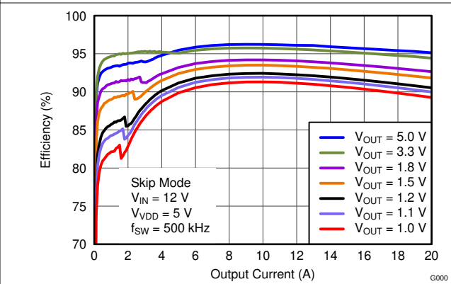
Figure 6-31. Efficiency vs Output Current
